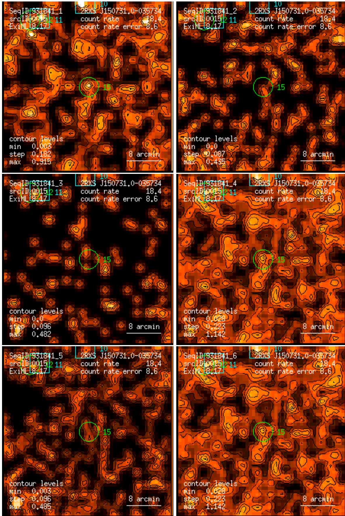
Figure 15: RASS 931841: detection 0015: band rate images, Gaussian filter: (1) PSPC channels 11 – 41, (2) 52 – 90, (3) 91 – 201, (4) 11 – 235, (5) 52 – 201, (6) 11 – 201. Broad band rates in counts/ks. Band rate contour levels in counts/ks/arcmin 2 .
