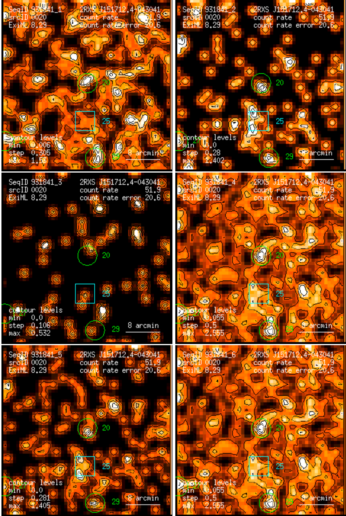
Figure 20: RASS 931841: detection 0020: band rate images, Gaussian filter: (1) PSPC channels 11 – 41, (2) 52 – 90, (3) 91 – 201, (4) 11 – 235, (5) 52 – 201, (6) 11 – 201. Broad band rates in counts/ks. Band rate contour levels in counts/ks/arcmin 2 .
