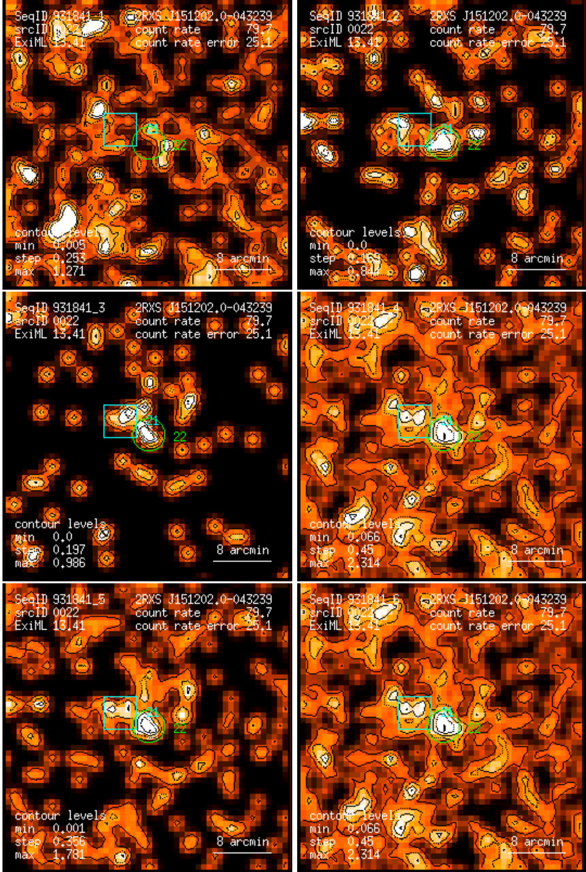
Figure 22: RASS 931841: detection 0022: band rate images, Gaussian filter: (1) PSPC channels 11 – 41, (2) 52 – 90, (3) 91 – 201, (4) 11 – 235, (5) 52 – 201, (6) 11 – 201. Broad band rates in counts/ks. Band rate contour levels in counts/ks/arcmin 2 .
