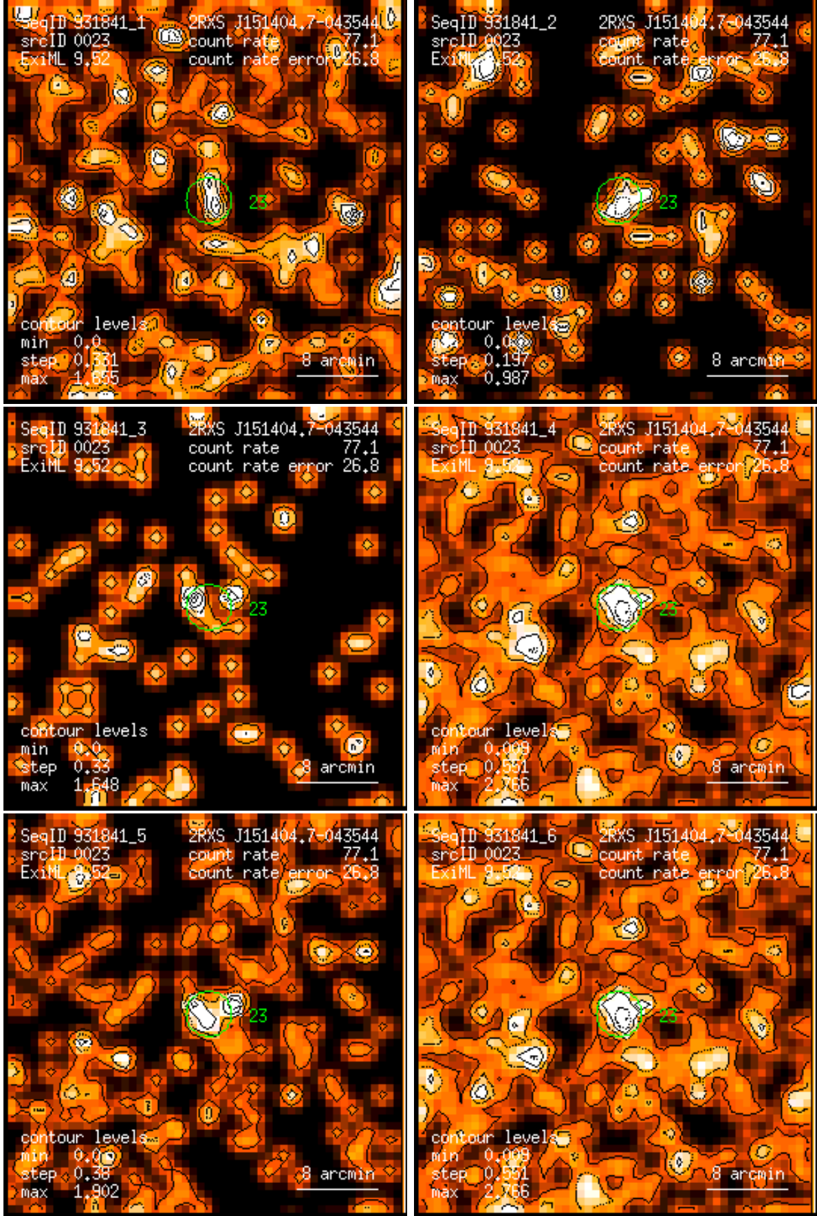
Figure 23: RASS 931841: detection 0023: band rate images, Gaussian filter: (1) PSPC channels 11 – 41, (2) 52 – 90, (3) 91 – 201, (4) 11 – 235, (5) 52 – 201, (6) 11 – 201. Broad band rates in counts/ks. Band rate contour levels in counts/ks/arcmin 2 .
