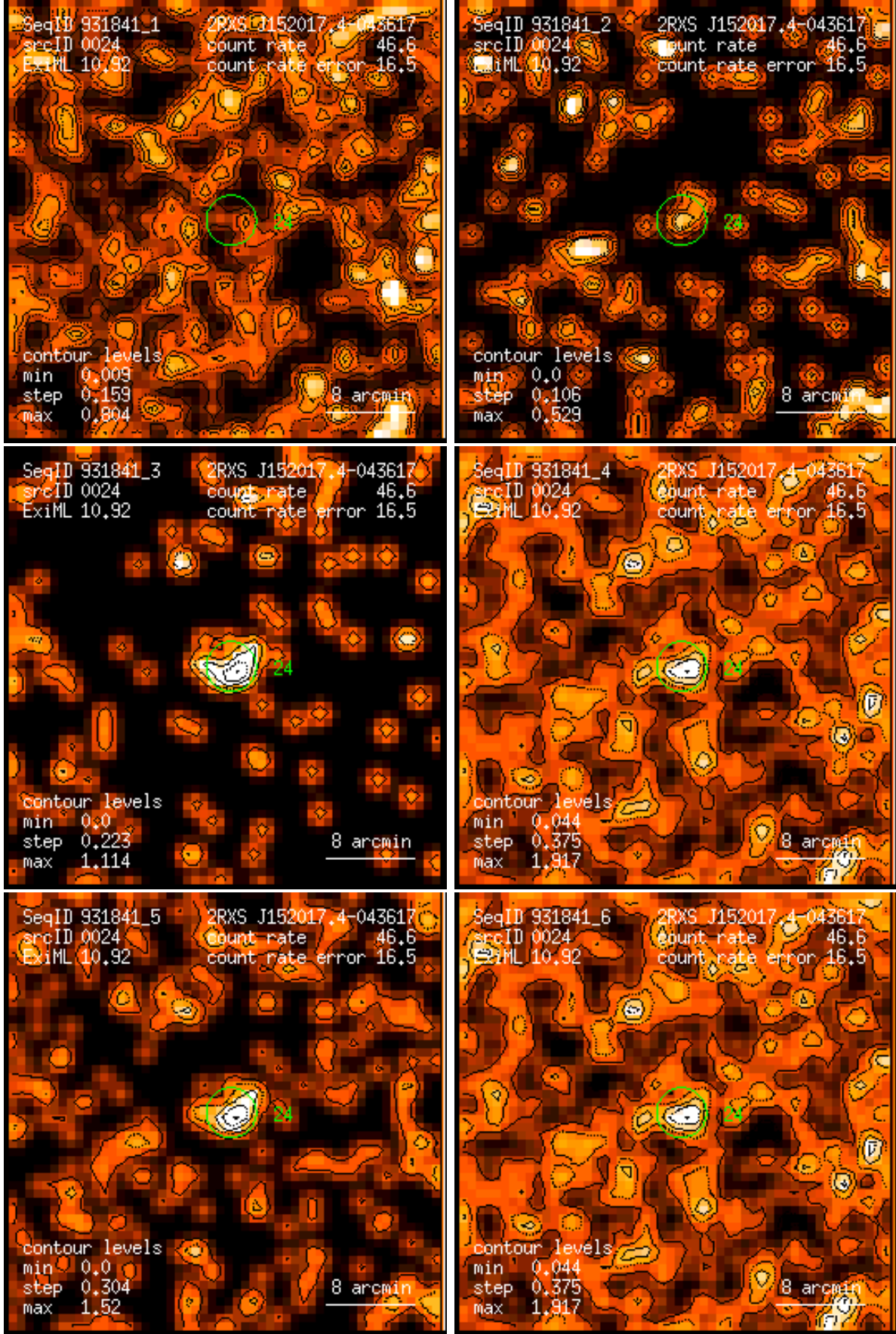
Figure 24: RASS 931841: detection 0024: band rate images, Gaussian filter: (1) PSPPC channels 11 – 41, (2) 52 – 90, (3) 91 – 201, (4) 11 – 235, (5) 52 – 201, (6) 11 – 201. Broad band rates in counts/ks. Band rate contour levels in counts/ks/arcmin 2 .
