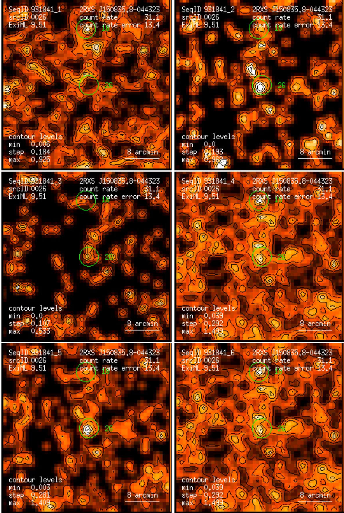
Figure 26: RASS 931841: detection 0026: band rate images, Gaussian filter: (1) PSPC channels 11 – 41, (2) 52 – 90, (3) 91 – 201, (4) 11 – 235, (5) 52 – 201, (6) 11 – 201. Broad band rates in counts/ks. Band rate contour levels in counts/ks/arcmin 2 .
