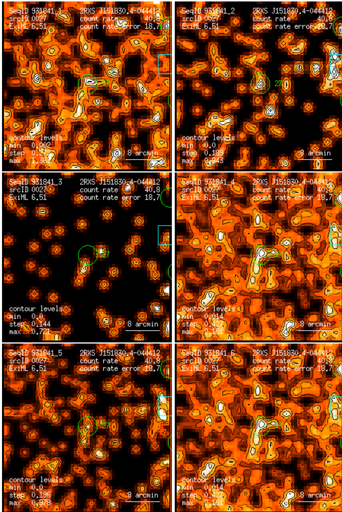
Figure 27: RASS 931841: detection 0027: band rate images, Gaussian filter: (1) PSPC channels 11 – 41, (2) 52 – 90, (3) 91 – 201, (4) 11 – 235, (5) 52 – 201, (6) 11 – 201. Broad band rates in counts/ks. Band rate contour levels in counts/ks/arcmin 2 .
