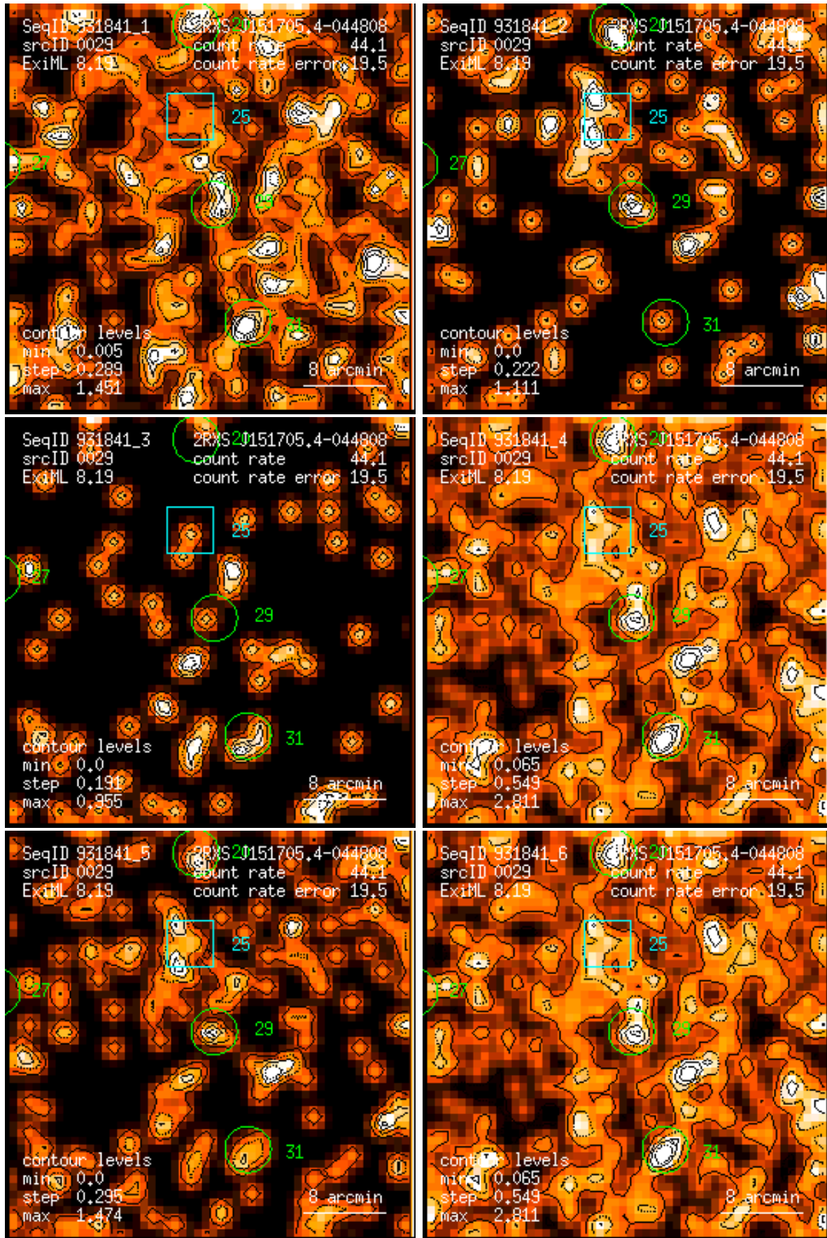
Figure 29: RASS 931841: detection 0029: band rate images, Gaussian filter: (1) PSPC channels 11 – 41, (2) 52 – 90, (3) 91 – 201, (4) 11 – 235, (5) 52 – 201, (6) 11 – 201. Broad band rates in counts/ks. Band rate contour levels in counts/ks/arcmin 2 .
