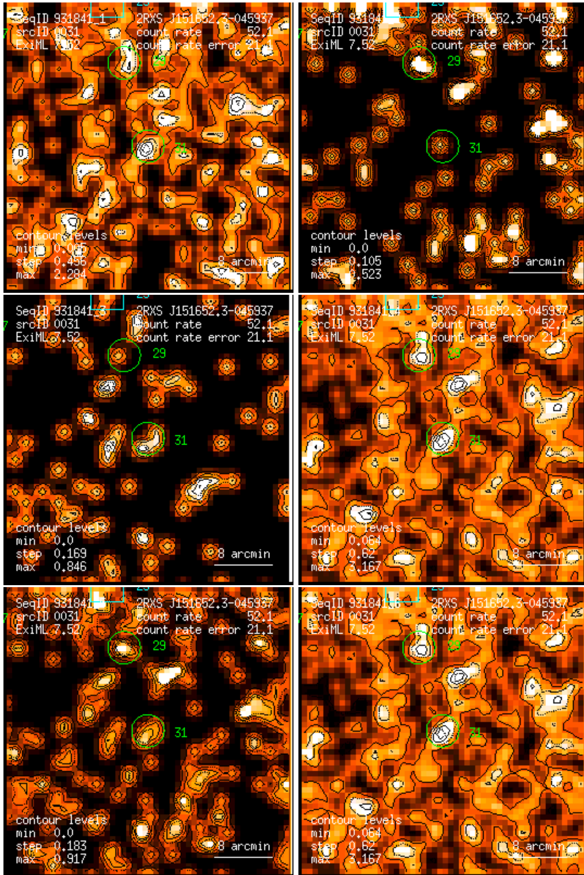
Figure 31: RASS 931841: detection 0031: band rate images, Gaussian filter: (1) PSPC channels 11 – 41, (2) 52 – 90, (3) 91 – 201, (4) 11 – 235, (5) 52 – 201, (6) 11 – 201. Broad band rates in counts/ks. Band rate contour levels in counts/ks/arcmin 2 .
