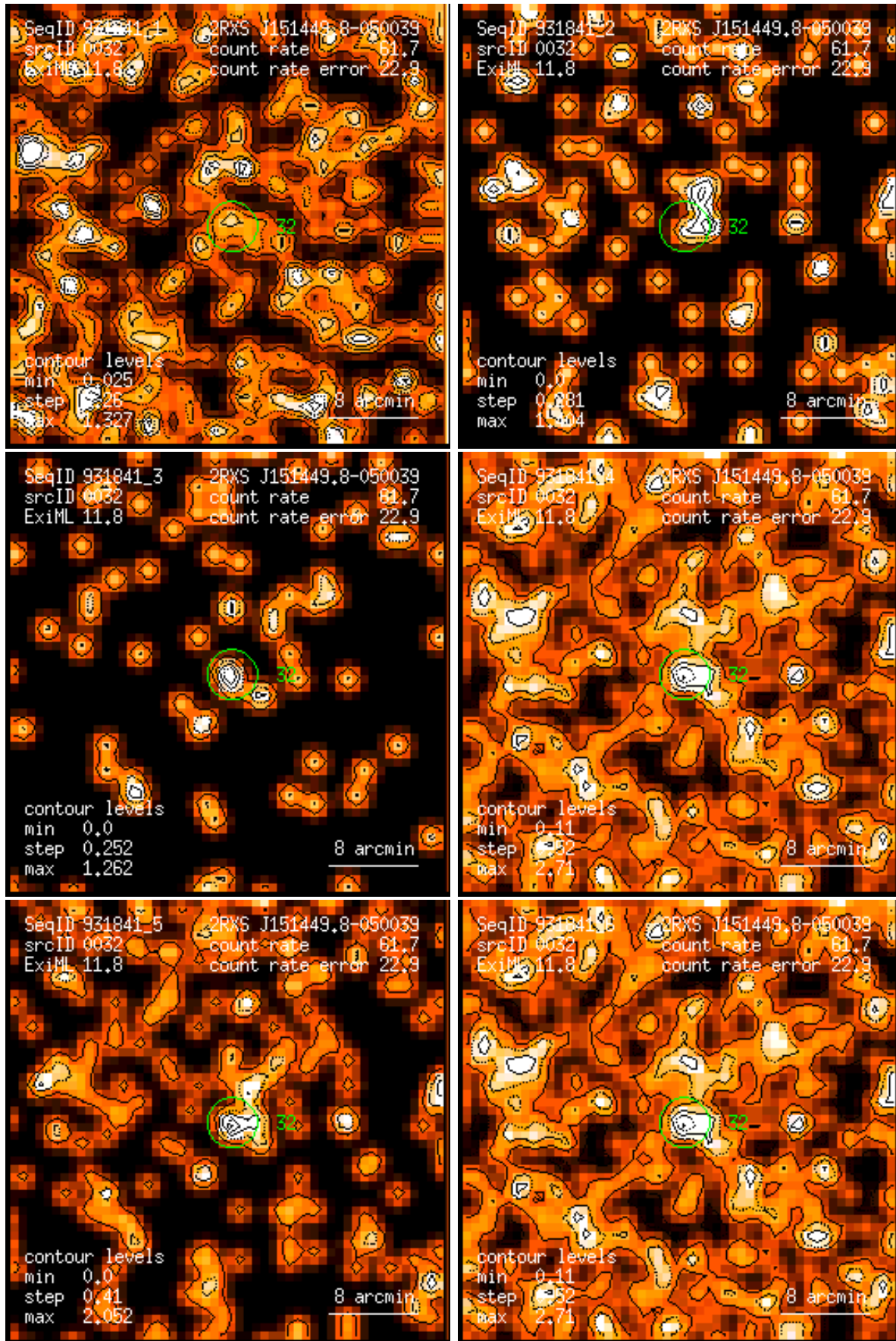
Figure 32: RASS 931841: detection 0032: band rate images, Gaussian filter: (1) PSPC channels 11 – 41, (2) 52 – 90, (3) 91 – 201, (4) 11 – 235, (5) 52 – 201, (6) 11 – 201. Broad band rates in counts/ks. Band rate contour levels in counts/ks/arcmin 2 .
