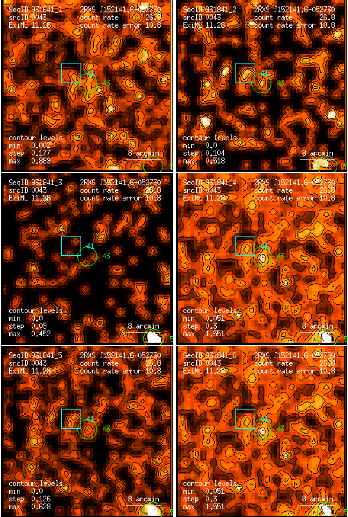
Figure 43: RASS 931841: detection 0043: band rate images, Gaussian filter: (1) PSPC channels 11 – 41, (2) 52 – 90, (3) 91 – 201, (4) 11 – 235, (5) 52 – 201, (6) 11 – 201. Broad band rates in counts/ks. Band rate contour levels in counts/ks/arcmin 2 .
