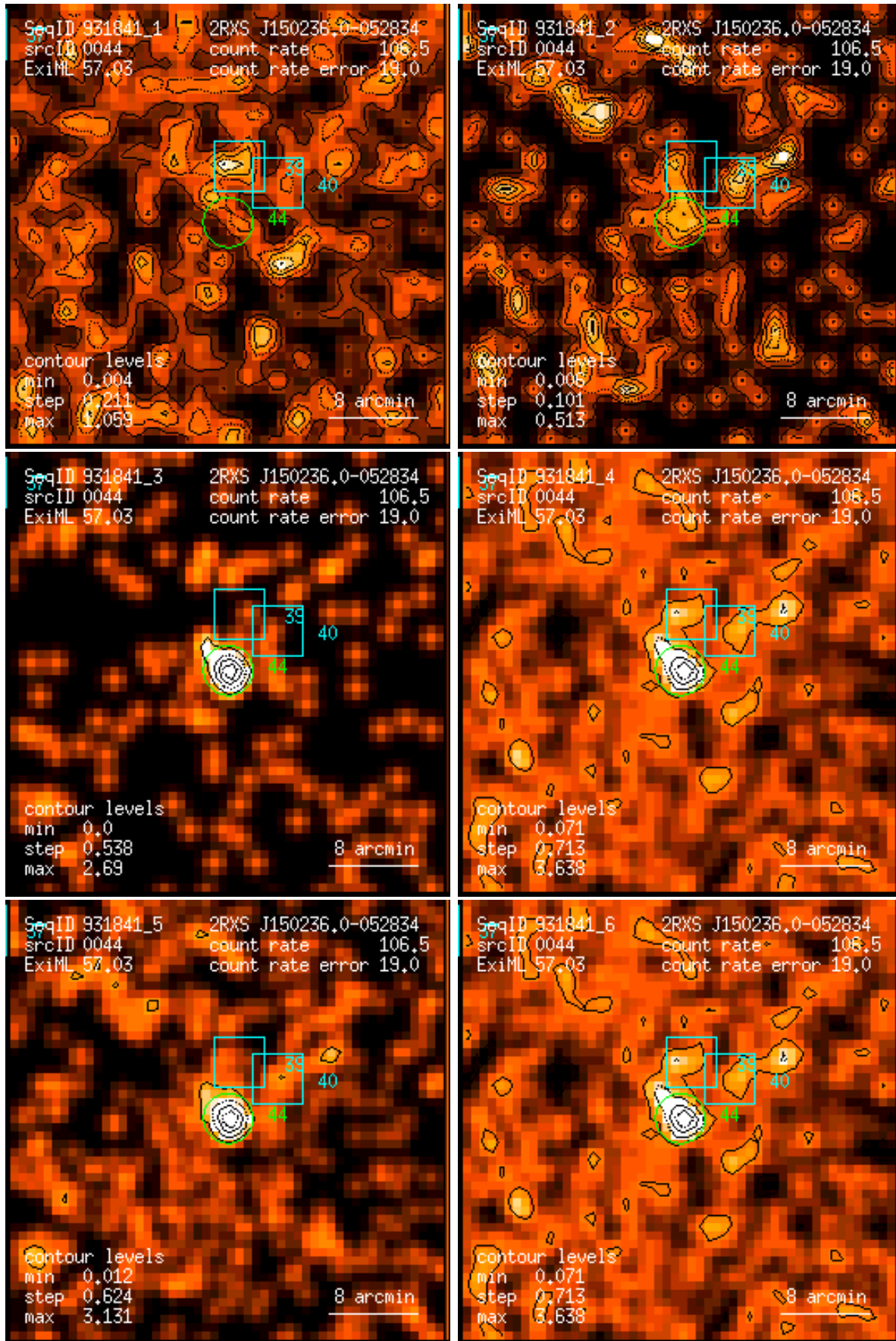
Figure 44: RASS 931841: detection 0044: band rate images, Gaussian filter: (1) PSPC channels 11 – 41, (2) 52 – 90, (3) 91 – 201, (4) 11 – 235, (5) 52 – 201, (6) 11 – 201. Broad band rates in counts/ks. Band rate contour levels in counts/ks/arcmin 2 .
