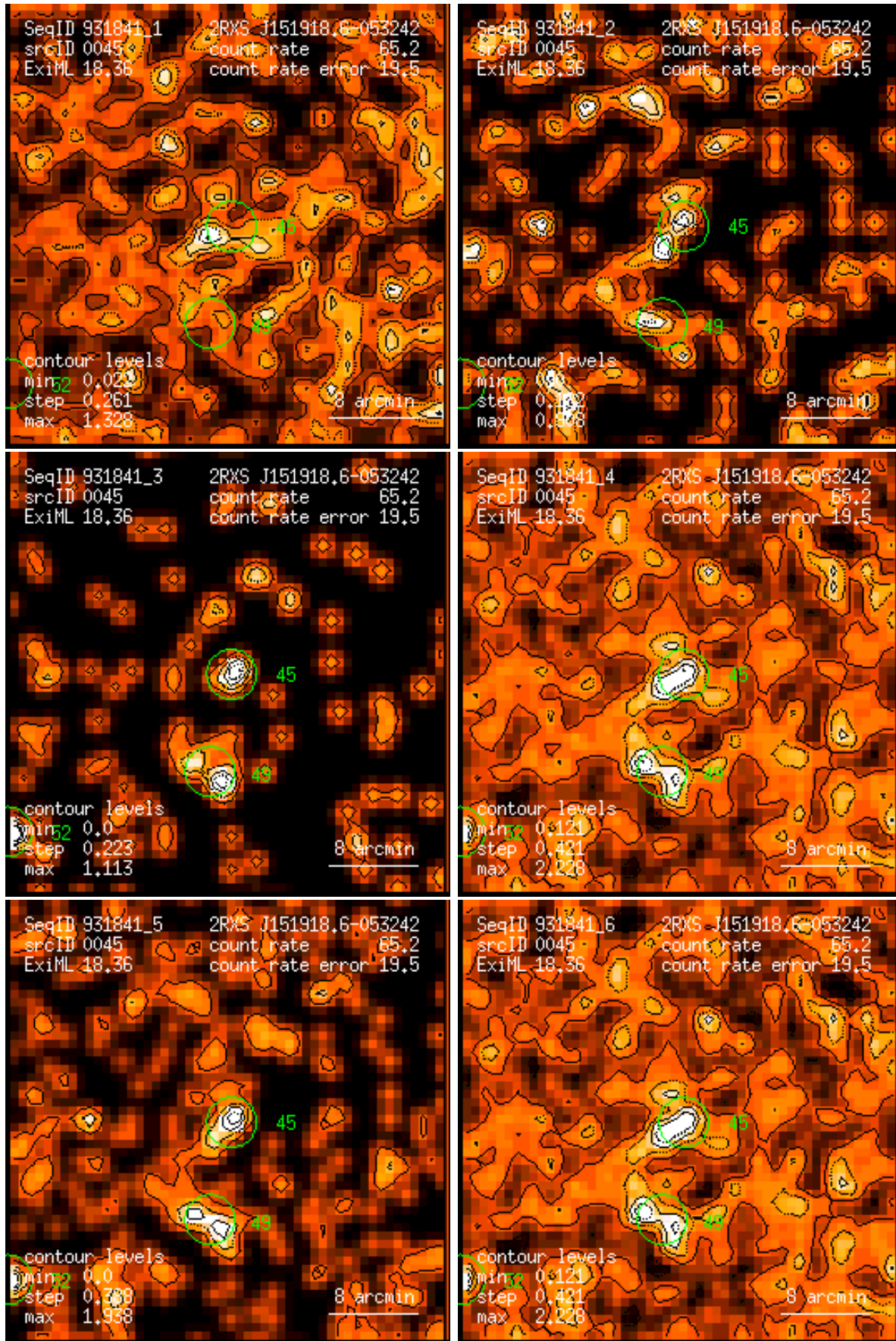
Figure 45: RASS 931841: detection 0045: band rate images, Gaussian filter: (1) PSPC channels 11 – 41, (2) 52 – 90, (3) 91 – 201, (4) 11 – 235, (5) 52 – 201, (6) 11 – 201. Broad band rates in counts/ks. Band rate contour levels in counts/ks/arcmin 2 .
