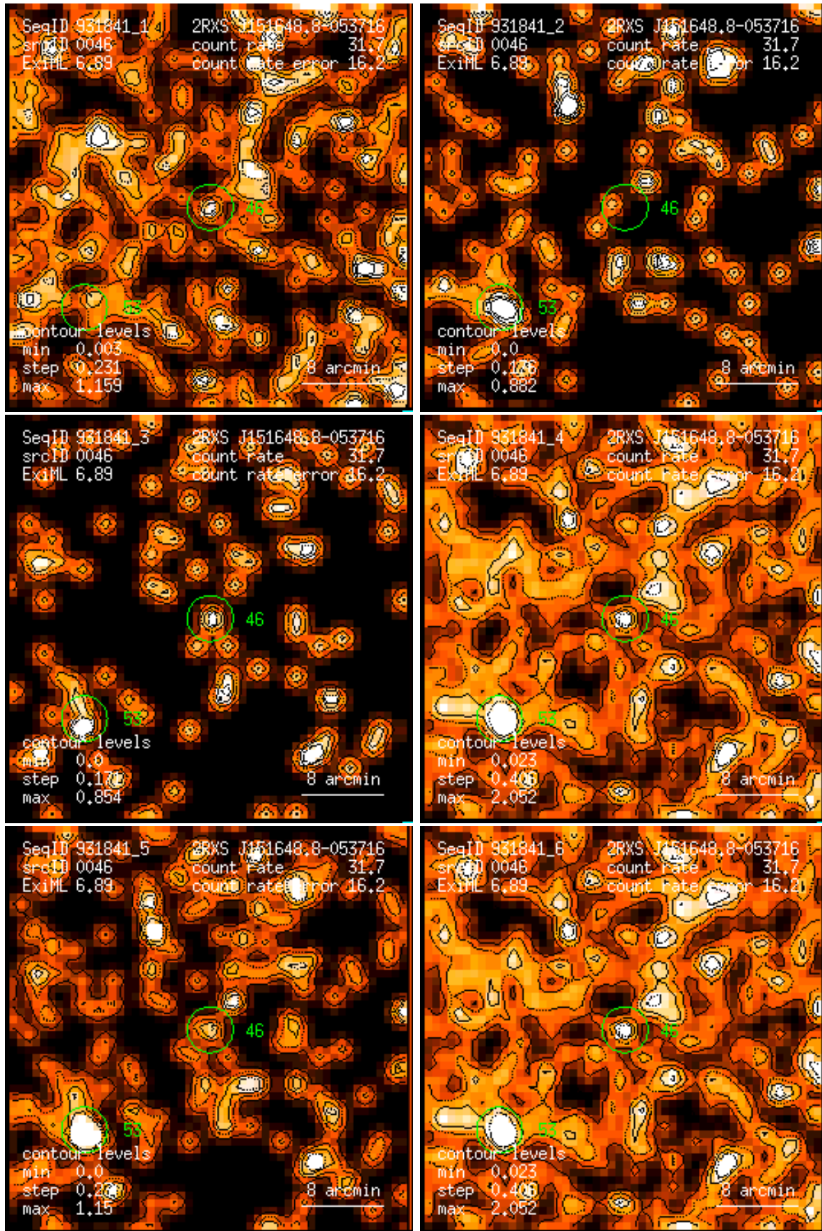
Figure 46: RASS 931841: detection 0046: band rate images, Gaussian filter: (1) PSPC channels 11 – 41, (2) 52 – 90, (3) 91 – 201, (4) 11 – 235, (5) 52 – 201, (6) 11 – 201. Broad band rates in counts/ks. Band rate contour levels in counts/ks/arcmin 2 .
