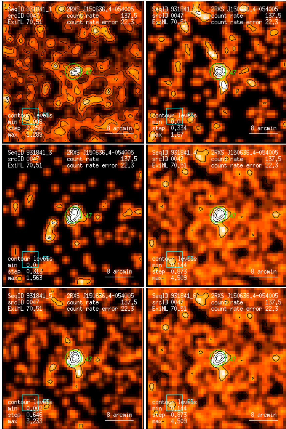
Figure 47: RASS 931841: detection 0047: band rate images, Gaussian filter: (1) PSPC channels 11 – 41, (2) 52 – 90, (3) 91 – 201, (4) 11 – 235, (5) 52 – 201, (6) 11 – 201. Broad band rates in counts/ks. Band rate contour levels in counts/ks/arcmin 2 .
