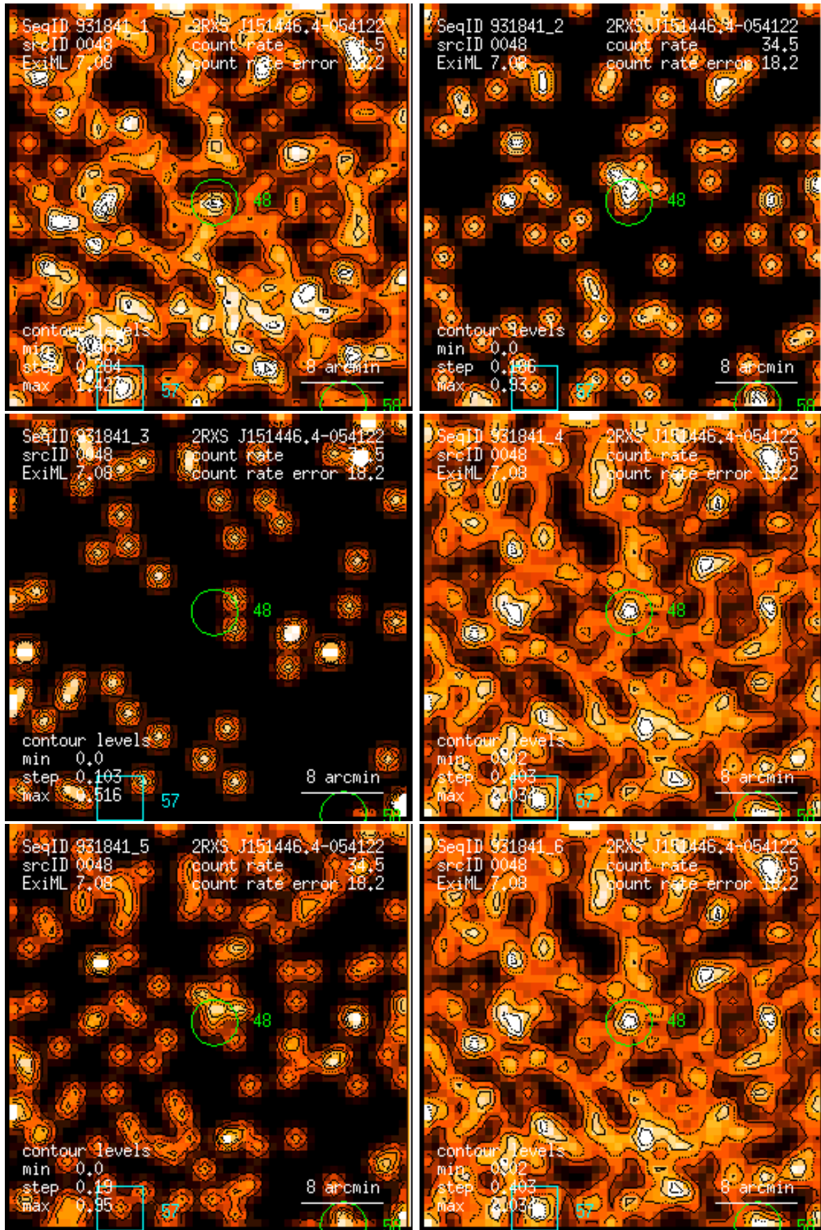
Figure 48: RASS 931841: detection 0048: band rate images, Gaussian filter: (1) PSPC channels 11 – 41, (2) 52 – 90, (3) 91 – 201, (4) 11 – 235, (5) 52 – 201, (6) 11 – 201. Broad band rates in counts/ks. Band rate contour levels in counts/ks/arcmin 2 .
