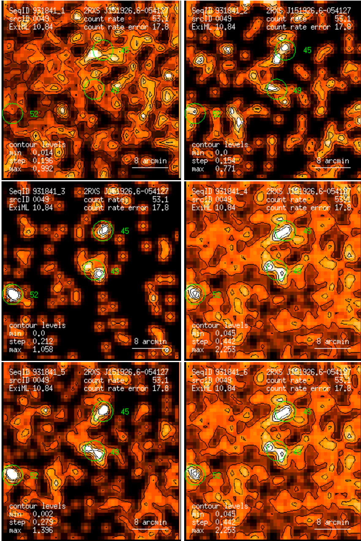
Figure 49: RASS 931841: detection 0049: band rate images, Gaussian filter: (1) PSPC channels 11 – 41, (2) 52 – 90, (3) 91 – 201, (4) 11 – 235, (5) 52 – 201, (6) 11 – 201. Broad band rates in counts/ks. Band rate contour levels in counts/ks/arcmin 2 .
