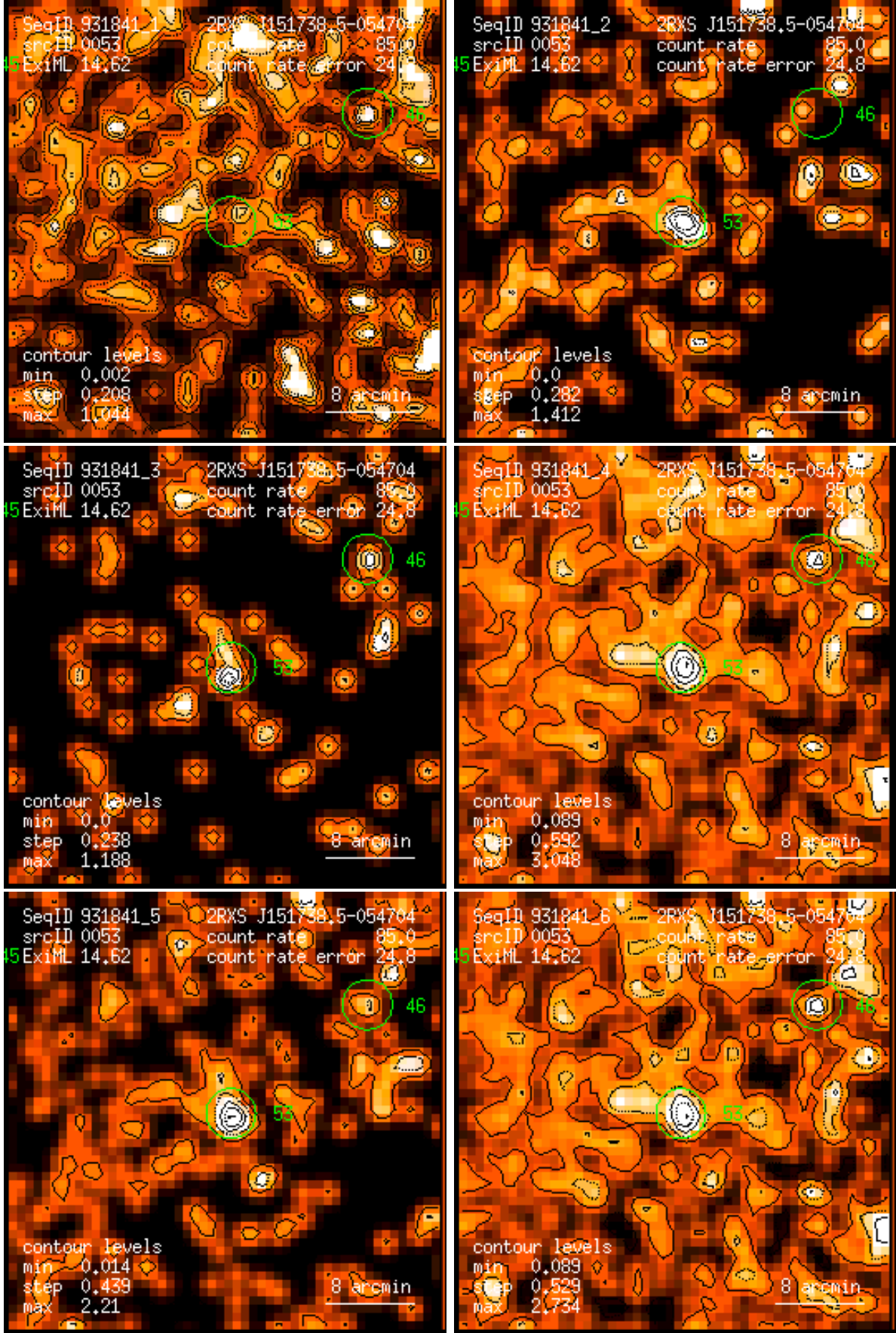
Figure 53: RASS 931841: detection 0053: band rate images, Gaussian filter: (1) PSPC channels 11 – 41, (2) 52 – 90, (3) 91 – 201, (4) 11 – 235, (5) 52 – 201, (6) 11 – 201. Broad band rates in counts/ks. Band rate contour levels in counts/ks/arcmin 2 .
