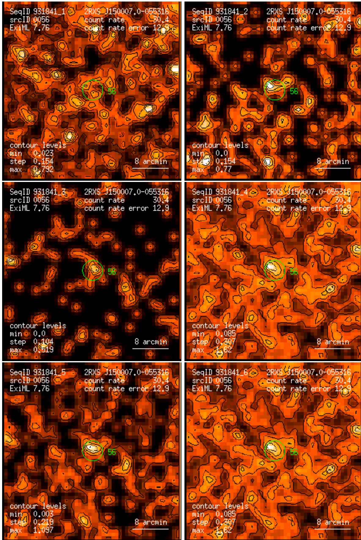
Figure 56: RASS 931841: detection 0056: band rate images, Gaussian filter: (1) PSPC channels 11 – 41, (2) 52 – 90, (3) 91 – 201, (4) 11 – 235, (5) 52 – 201, (6) 11 – 201. Broad band rates in counts/ks. Band rate contour levels in counts/ks/arcmin 2 .
