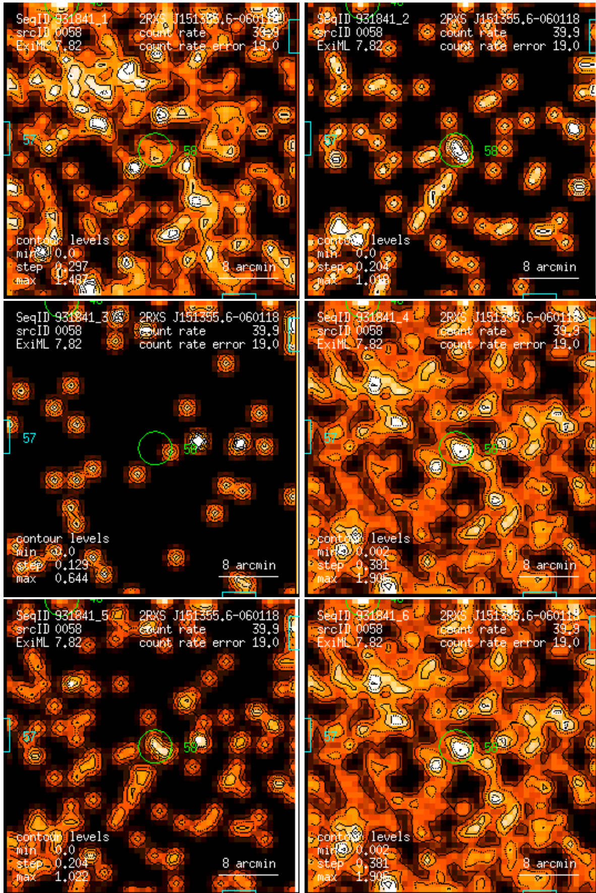
Figure 58: RASS 931841: detection 0058: band rate images, Gaussian filter: (1) PSPC channels 11 – 41, (2) 52 – 90, (3) 91 – 201, (4) 11 – 235, (5) 52 – 201, (6) 11 – 201. Broad band rates in counts/ks. Band rate contour levels in counts/ks/arcmin 2 .
