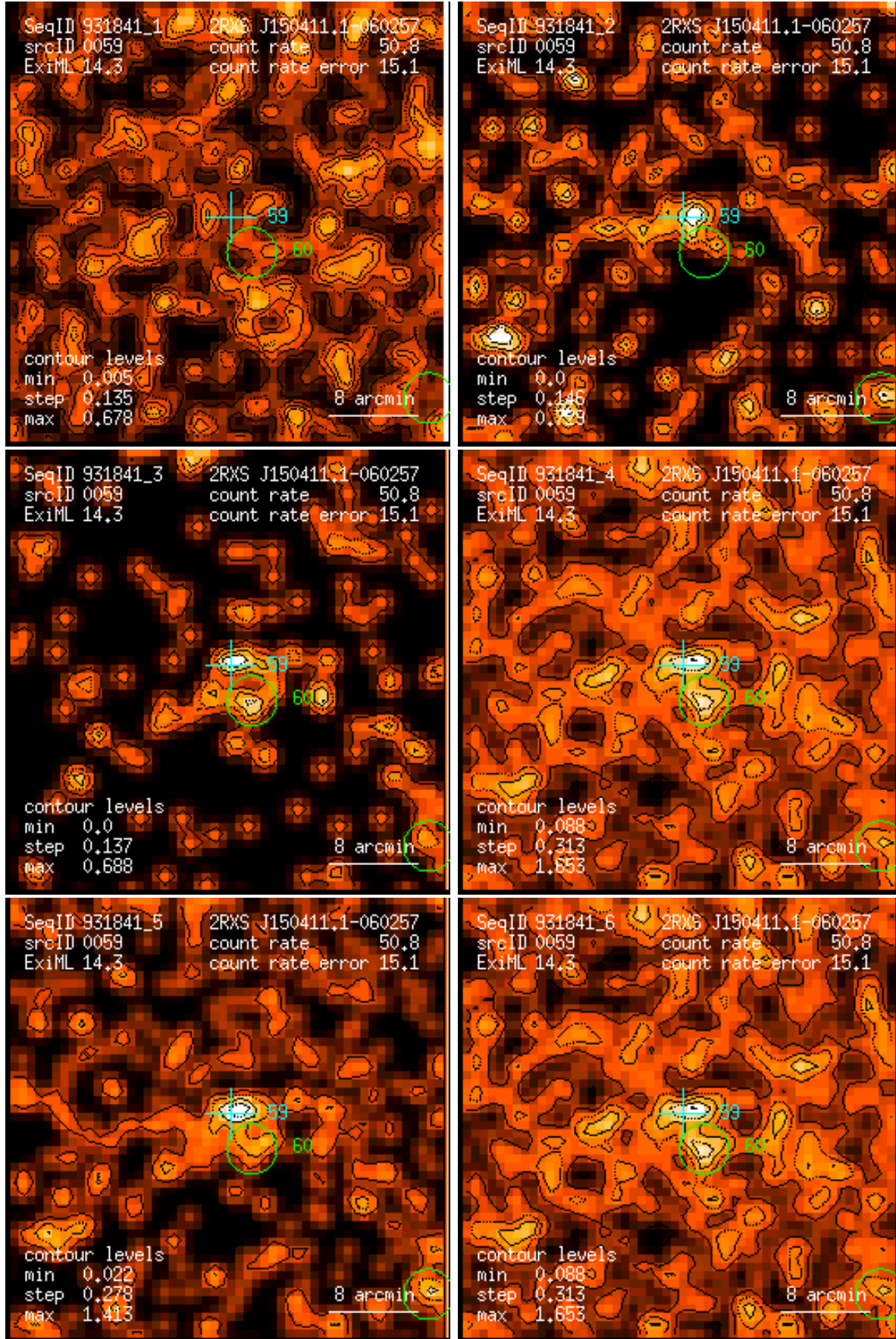
Figure 59: RASS 931841: detection 0059: band rate images, Gaussian filter: (1) PSPC channels 11 – 41, (2) 52 – 90, (3) 91 – 201, (4) 11 – 235, (5) 52 – 201, (6) 11 – 201. Broad band rates in counts/ks. Band rate contour levels in counts/ks/arcmin 2 .
