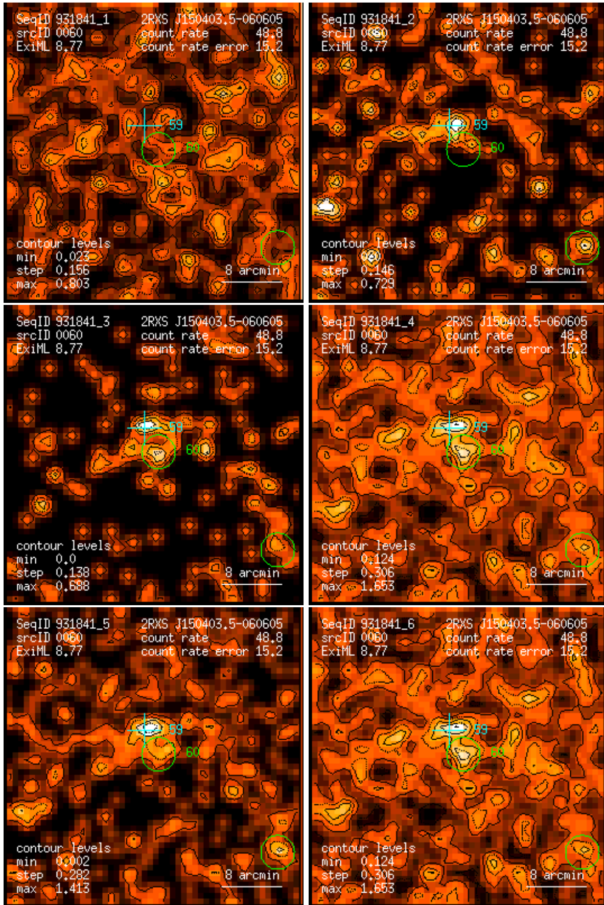
Figure 60: RASS 931841: detection 0060: band rate images, Gaussian filter: (1) PSPC channels 11 – 41, (2) 52 – 90, (3) 91 – 201, (4) 11 – 235, (5) 52 – 201, (6) 11 – 201. Broad band rates in counts/ks. Band rate contour levels in counts/ks/arcmin 2 .
