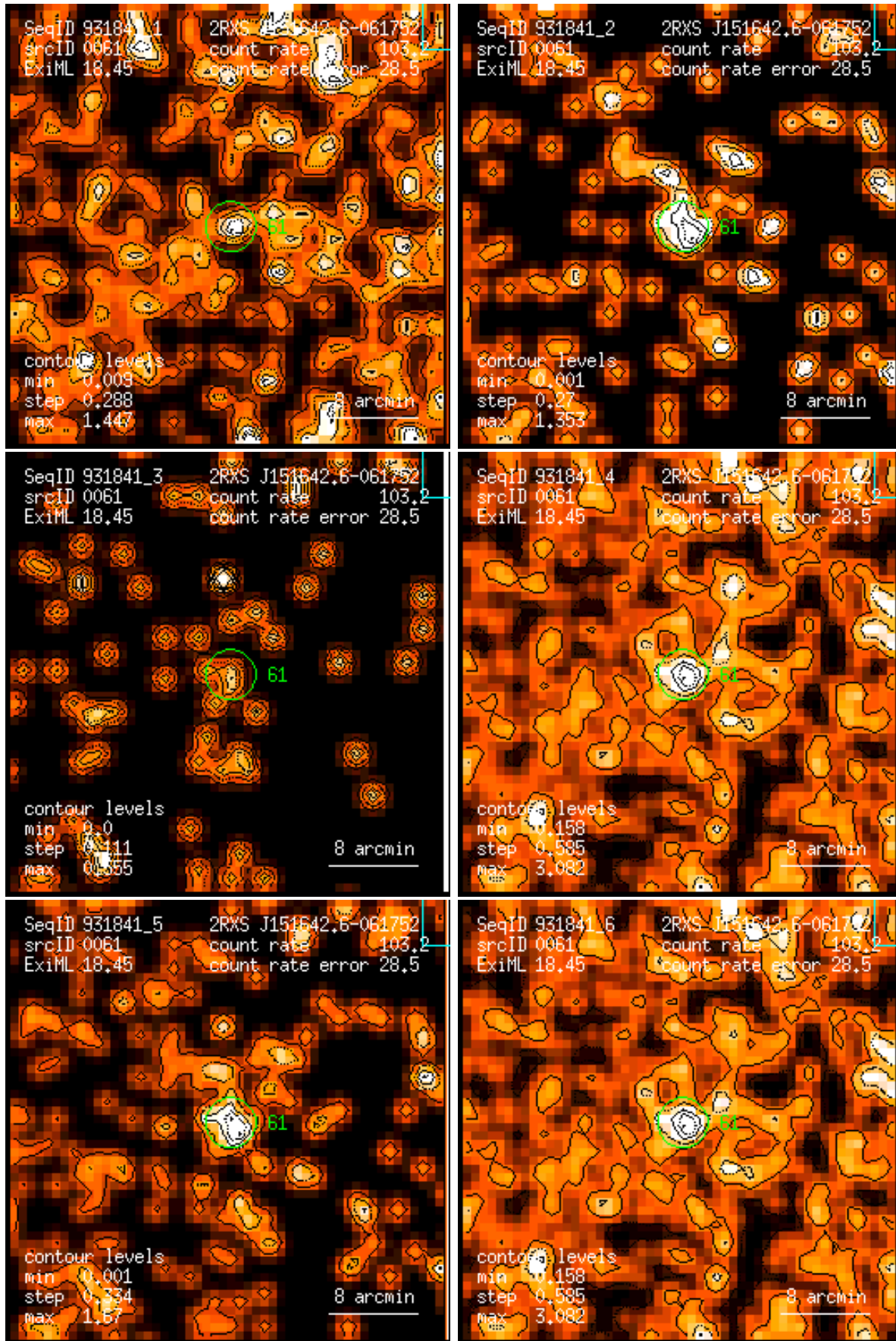
Figure 61: RASS 931841: detection 0061: band rate images, Gaussian filter: (1) PSPC channels 11 – 41, (2) 52 – 90, (3) 91 – 201, (4) 11 – 235, (5) 52 – 201, (6) 11 – 201. Broad band rates in counts/ks. Band rate contour levels in counts/ks/arcmin 2 .
