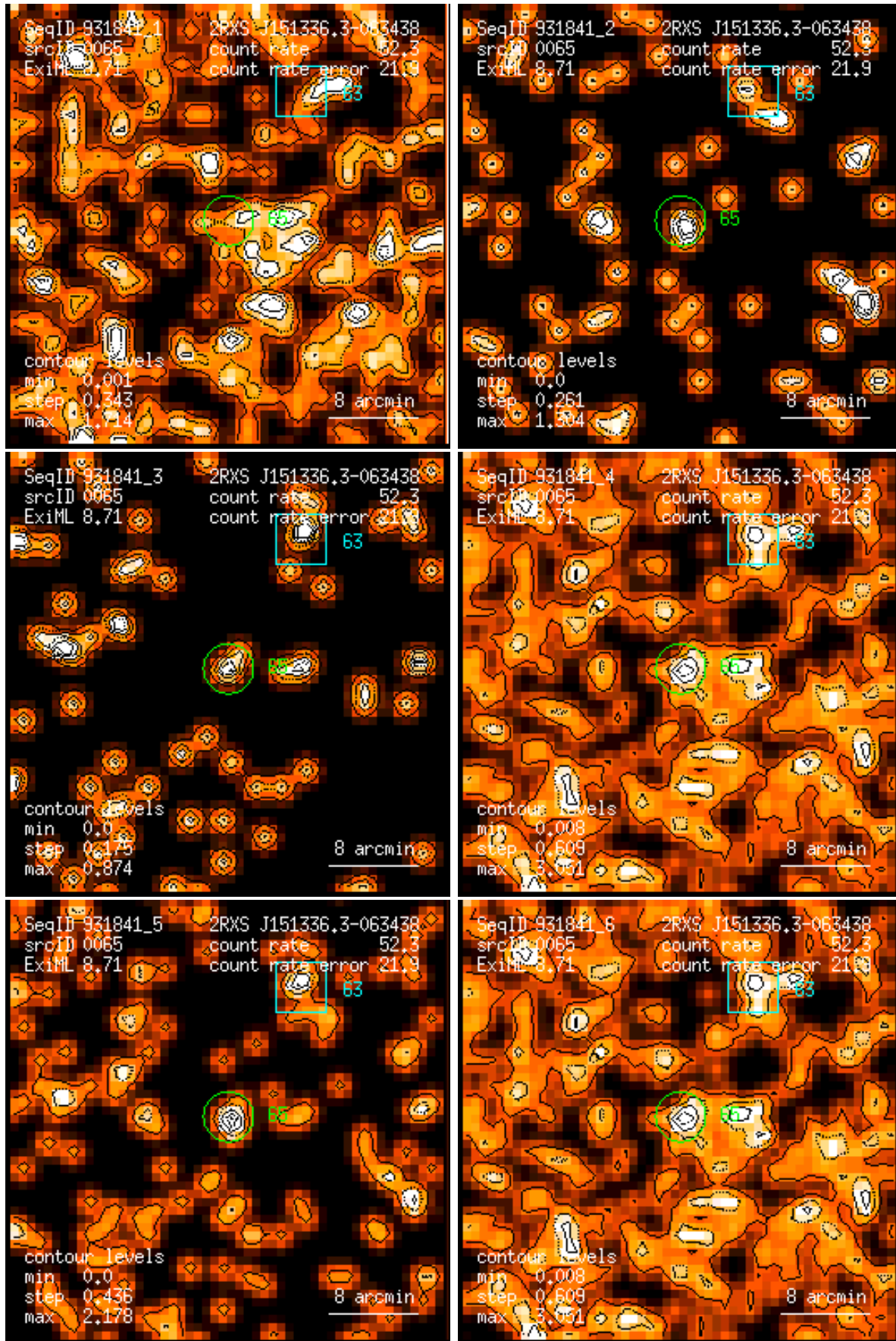
Figure 65: RASS 931841: detection 0065: band rate images, Gaussian filter: (1) PSPC channels 11 – 41, (2) 52 – 90, (3) 91 – 201, (4) 11 – 235, (5) 52 – 201, (6) 11 – 201. Broad band rates in counts/ks. Band rate contour levels in counts/ks/arcmin 2 .
