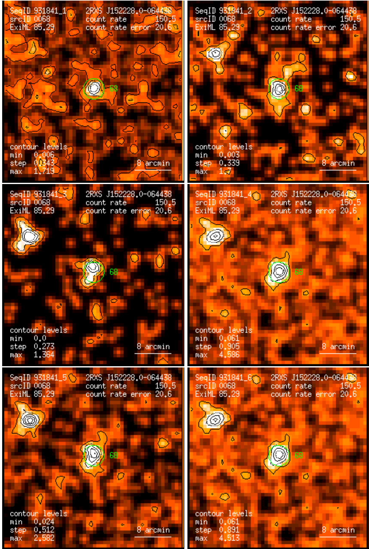
Figure 68: RASS 931841: detection 0068: band rate images, Gaussian filter: (1) PSPC channels 11 – 41, (2) 52 – 90, (3) 91 – 201, (4) 11 – 235, (5) 52 – 201, (6) 11 – 201. Broad band rates in counts/ks. Band rate contour levels in counts/ks/arcmin 2 .
