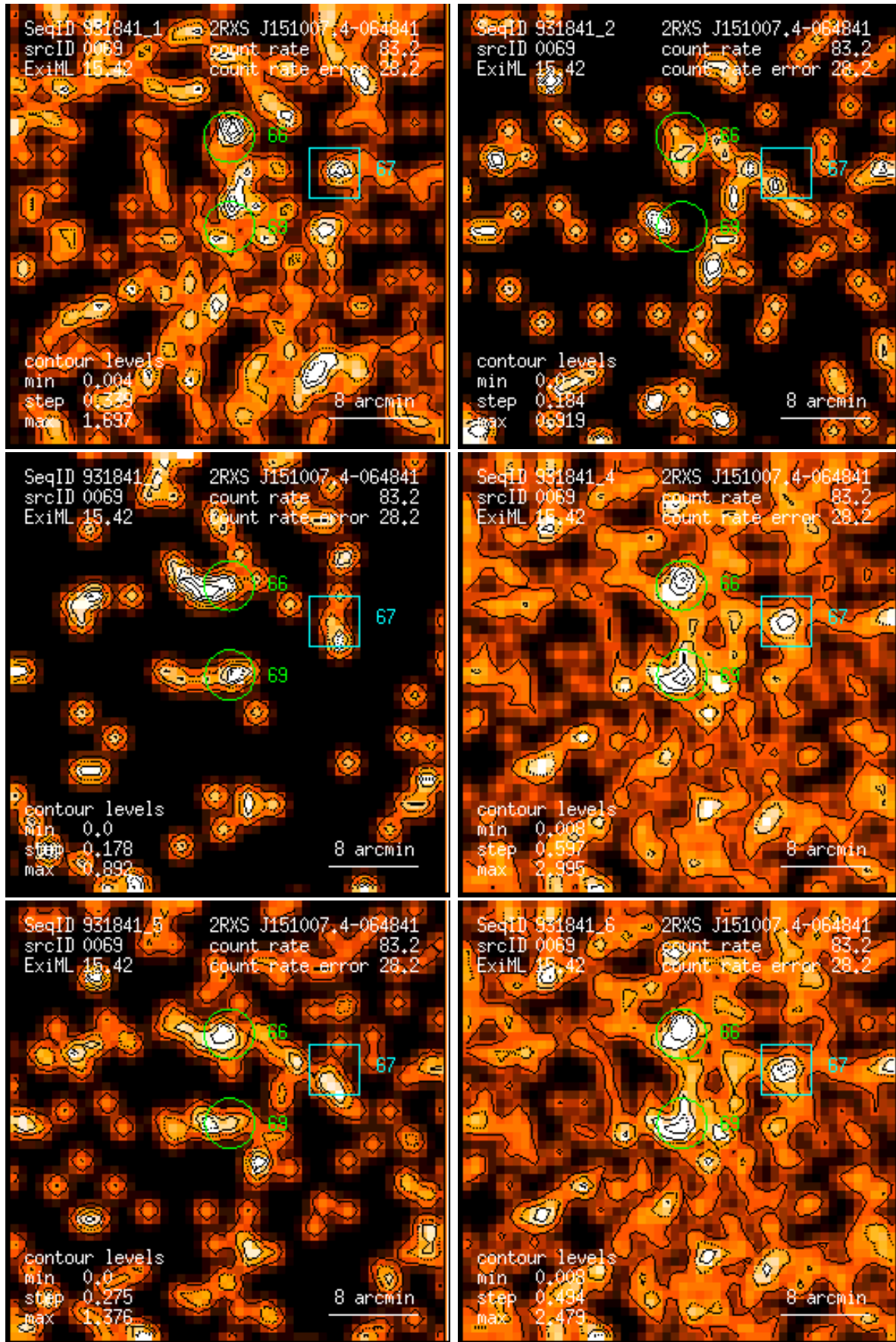
Figure 69: RASS 931841: detection 0069: band rate images, Gaussian filter: (1) PSPC channels 11 – 41, (2) 52 – 90, (3) 91 – 201, (4) 11 – 235, (5) 52 – 201, (6) 11 – 201. Broad band rates in counts/ks. Band rate contour levels in counts/ks/arcmin 2 .
