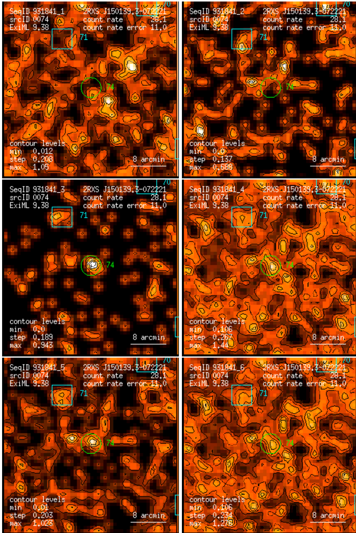
Figure 74: RASS 931841: detection 0074: band rate images, Gaussian filter: (1) PSPC channels 11 – 41, (2) 52 – 90, (3) 91 – 201, (4) 11 – 235, (5) 52 – 201, (6) 11 – 201. Broad band rates in counts/ks. Band rate contour levels in counts/ks/arcmin 2 .
