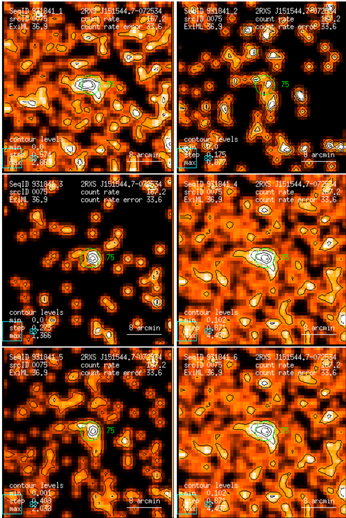
Figure 75: RASS 931841: detection 0075: band rate images, Gaussian filter: (1) PSPC channels 11 – 41, (2) 52 – 90, (3) 91 – 201, (4) 11 – 235, (5) 52 – 201, (6) 11 – 201. Broad band rates in counts/ks. Band rate contour levels in counts/ks/arcmin 2 .
