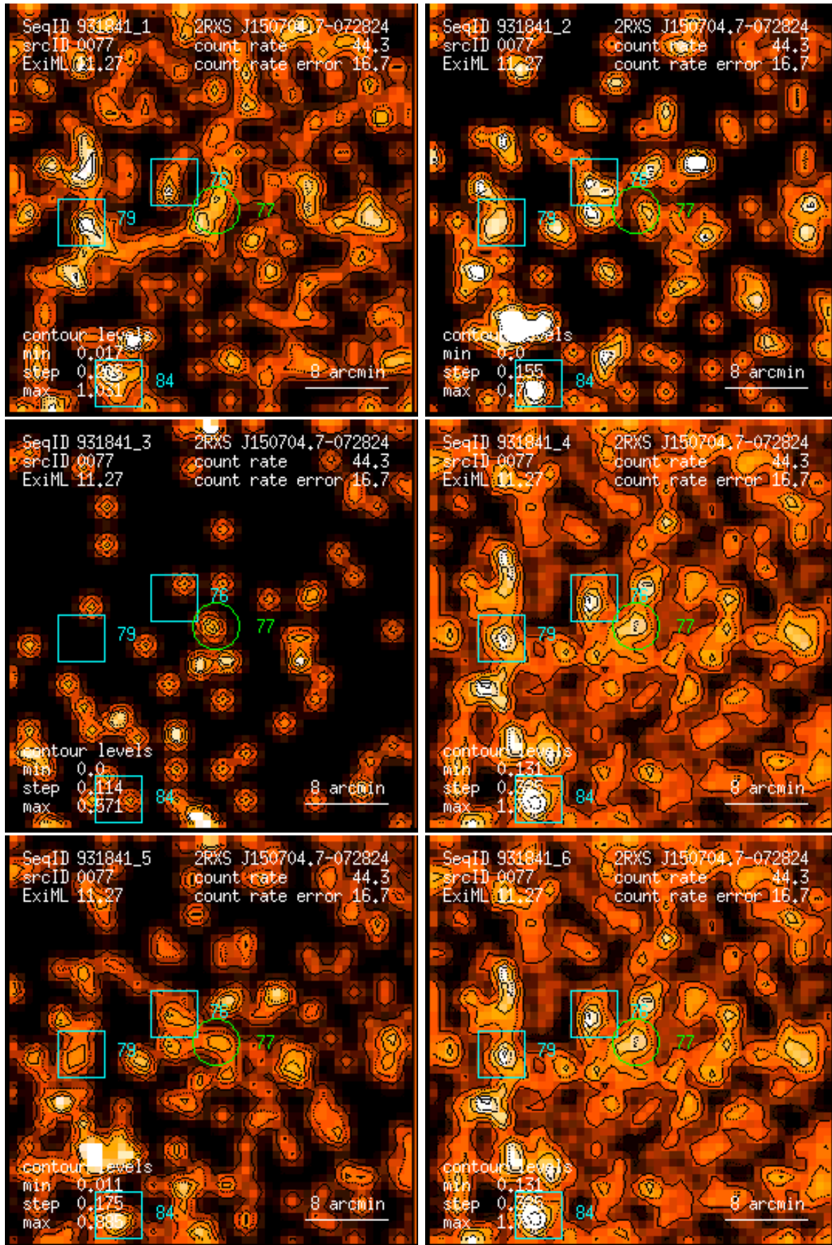
Figure 77: RASS 931841: detection 0077: band rate images, Gaussian filter: (1) PSPC channels 11 – 41, (2) 52 – 90, (3) 91 – 201, (4) 11 – 235, (5) 52 – 201, (6) 11 – 201. Broad band rates in counts/ks. Band rate contour levels in counts/ks/arcmin 2 .
