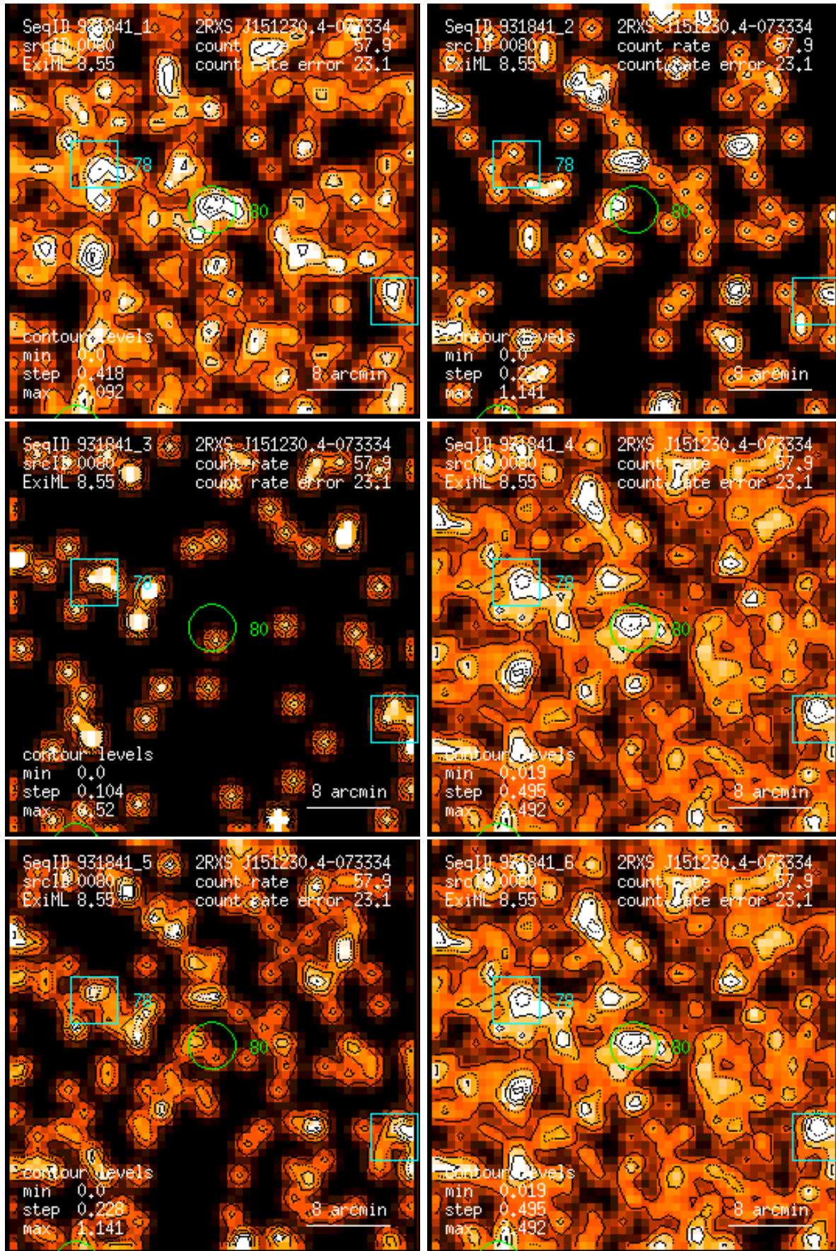
Figure 80: RASS 931841: detection 0080: band rate images, Gaussian filter: (1) PSPC channels 11 – 41, (2) 52 – 90, (3) 91 – 201, (4) 11 – 235, (5) 52 – 201, (6) 11 – 201. Broad band rates in counts/ks. Band rate contour levels in counts/ks/arcmin 2 .
