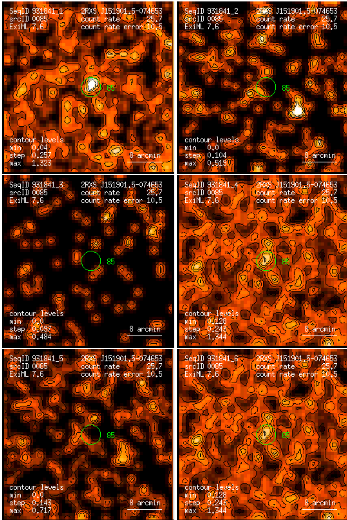
Figure 85: RASS 931841: detection 0085: band rate images, Gaussian filter: (1) PSPC channels 11 – 41, (2) 52 – 90, (3) 91 – 201, (4) 11 – 235, (5) 52 – 201, (6) 11 – 201. Broad band rates in counts/ks. Band rate contour levels in counts/ks/arcmin 2 .
