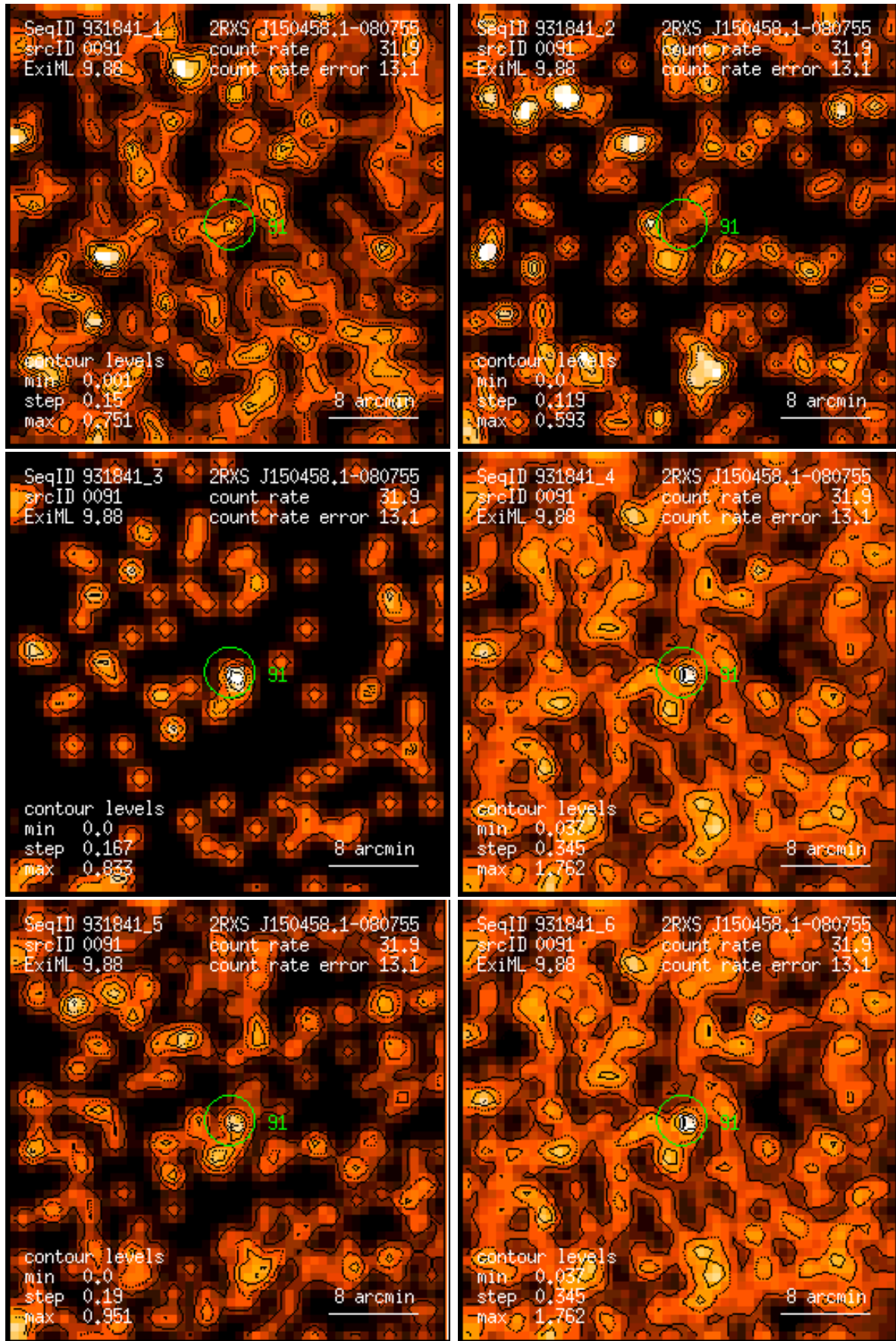
Figure 91: RASS 931841: detection 0091: band rate images, Gaussian filter: (1) PSPC channels 11 – 41, (2) 52 – 90, (3) 91 – 201, (4) 11 – 235, (5) 52 – 201, (6) 11 – 201. Broad band rates in counts/ks. Band rate contour levels in counts/ks/arcmin 2 .
