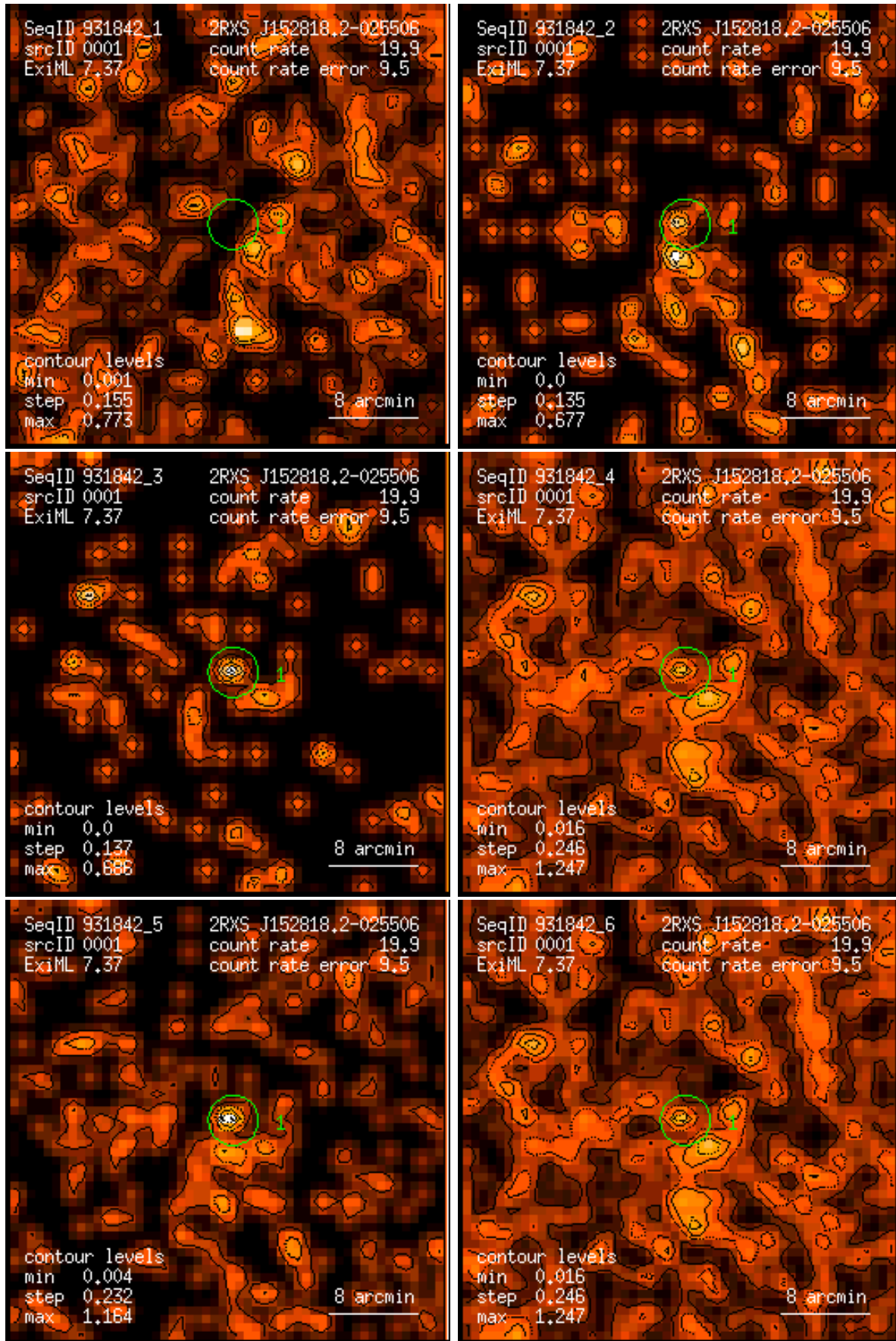
Figure 1: RASS 931842: detection 0001: band rate images, Gaussian filter: (1) PSPC channels 11 – 41, (2) 52 – 90, (3) 91 – 201, (4) 11 – 235, (5) 52 – 201, (6) 11 – 201. Broad band rates in counts/ks. Band rate contour levels in counts/ks/arcmin 2 .
