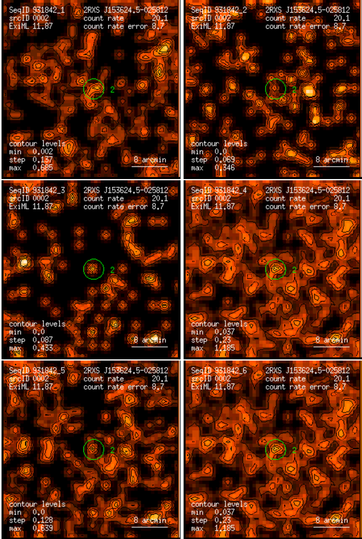
Figure 2: RASS 931842: detection 0002: band rate images, Gaussian filter: (1) PSPC channels 11 – 41, (2) 52 – 90, (3) 91 – 201, (4) 11 – 235, (5) 52 – 201, (6) 11 – 201. Broad band rates in counts/ks. Band rate contour levels in counts/ks/arcmin 2 .
