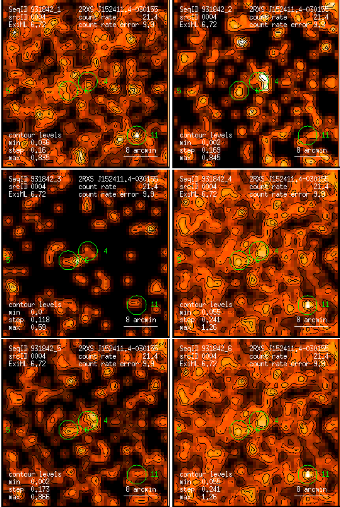
Figure 4: RASS 931842: detection 0004: band rate images, Gaussian filter: (1) PSPC channels 11 – 41, (2) 52 – 90, (3) 91 – 201, (4) 11 – 235, (5) 52 – 201, (6) 11 – 201. Broad band rates in counts/ks. Band rate contour levels in counts/ks/arcmin 2 .
