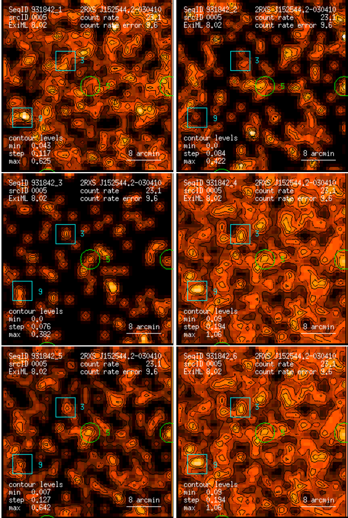
Figure 5: RASS 931842: detection 0005: band rate images, Gaussian filter: (1) PSPC channels 11 – 41, (2) 52 – 90, (3) 91 – 201, (4) 11 – 235, (5) 52 – 201, (6) 11 – 201. Broad band rates in counts/ks. Band rate contour levels in counts/ks/arcmin 2 .
