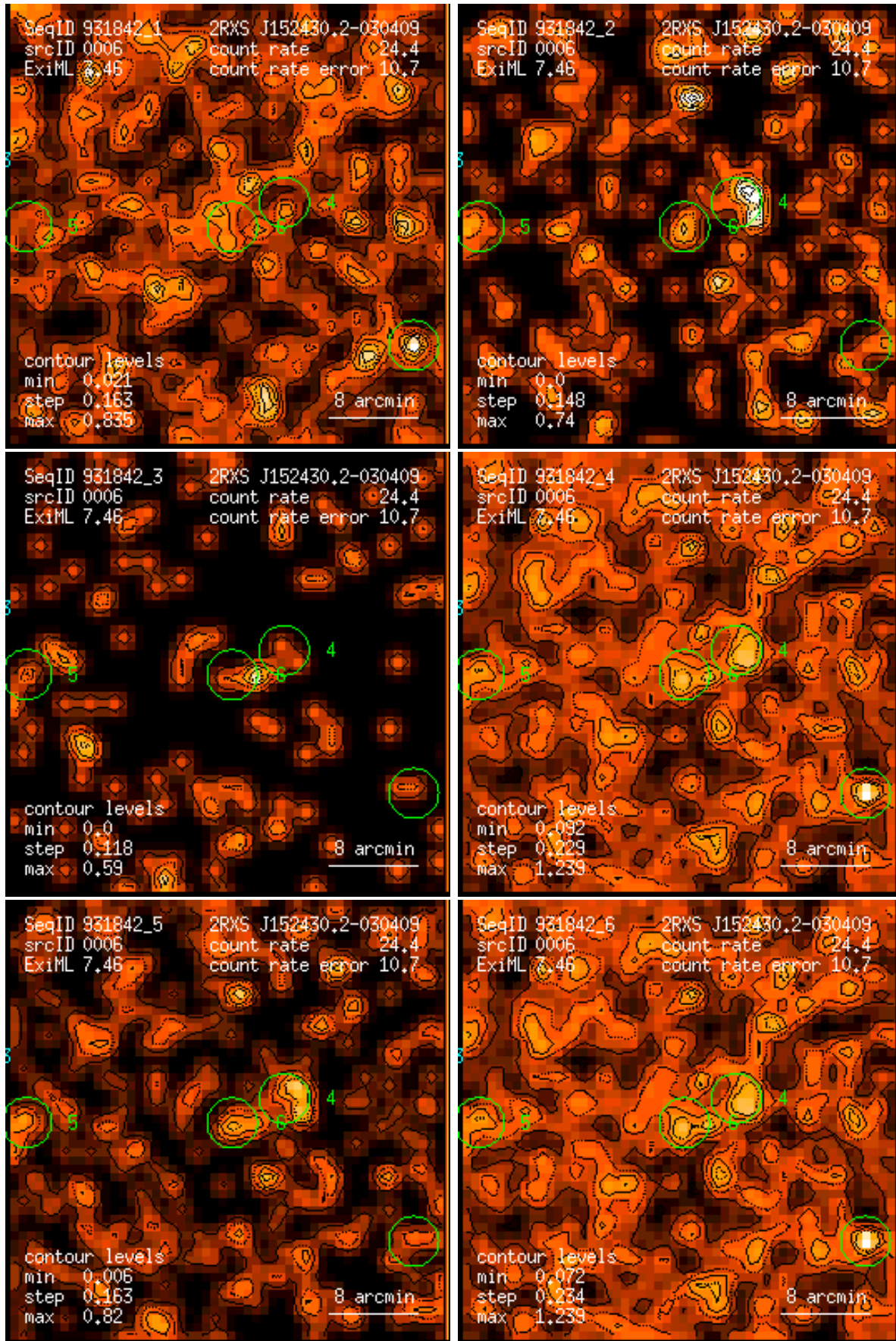
Figure 6: RASS 931842: detection 0006: band rate images, Gaussian filter: (1) PSPC channels 11 – 41, (2) 52 – 90, (3) 91 – 201, (4) 11 – 235, (5) 52 – 201, (6) 11 – 201. Broad band rates in counts/ks. Band rate contour levels in counts/ks/arcmin 2 .
