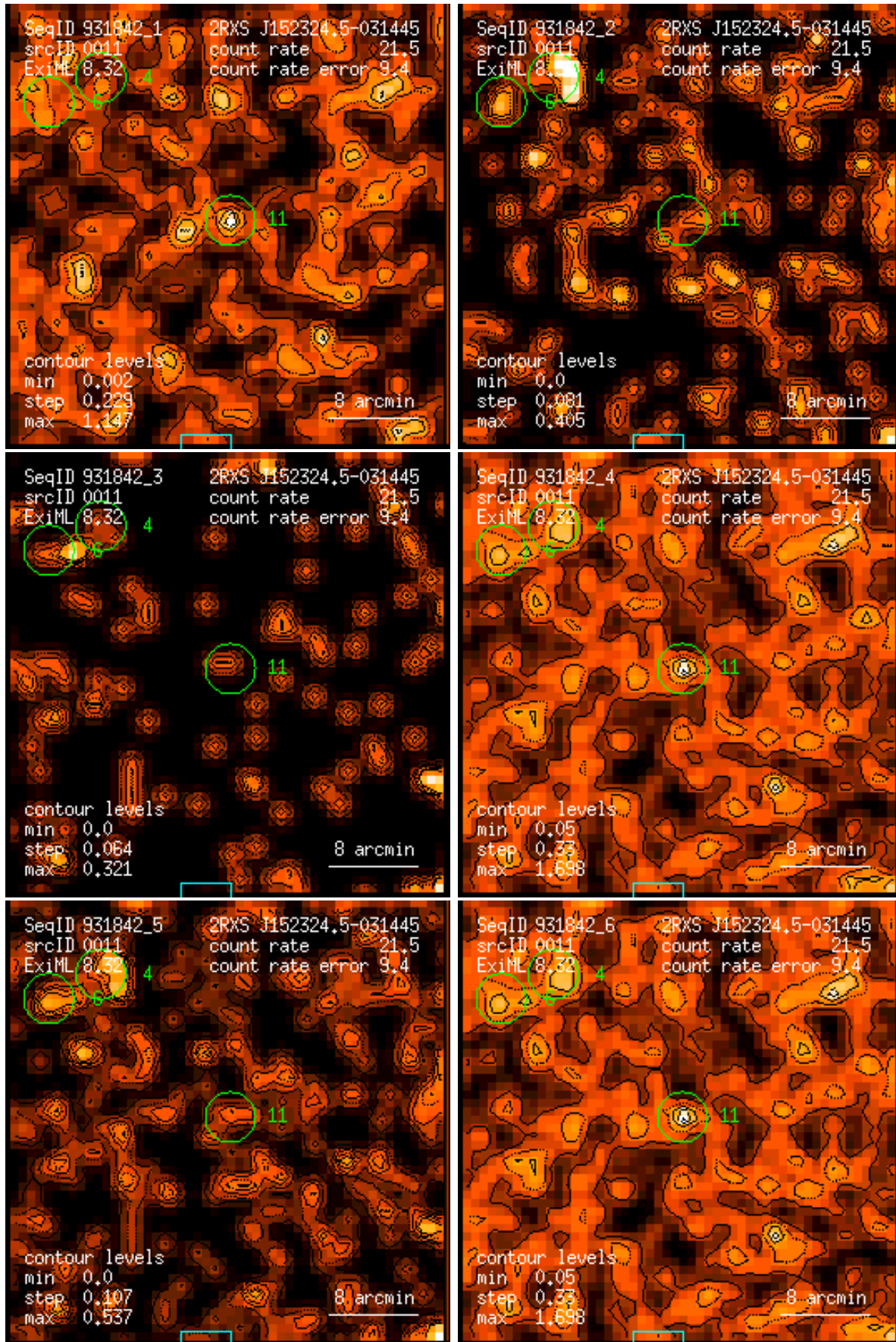
Figure 11: RASS 931842: detection 0011: band rate images, Gaussian filter: (1) PSPC channels 11 – 41, (2) 52 – 90, (3) 91 – 201, (4) 11 – 235, (5) 52 – 201, (6) 11 – 201. Broad band rates in counts/ks. Band rate contour levels in counts/ks/arcmin 2 .
