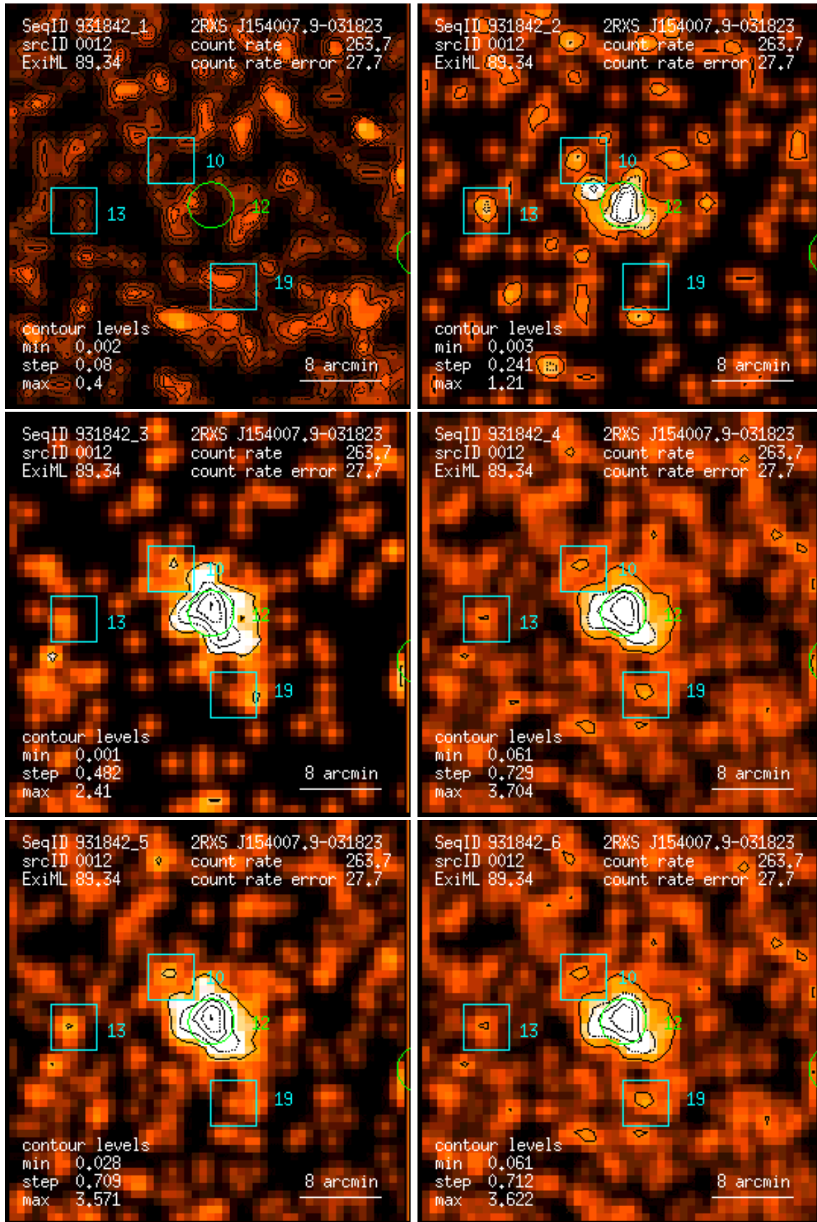
Figure 12: RASS 931842: detection 0012: band rate images, Gaussian filter: (1) PSPC channels 11 – 41, (2) 52 – 90, (3) 91 – 201, (4) 11 – 235, (5) 52 – 201, (6) 11 – 201. Broad band rates in counts/ks. Band rate contour levels in counts/ks/arcmin 2 .
