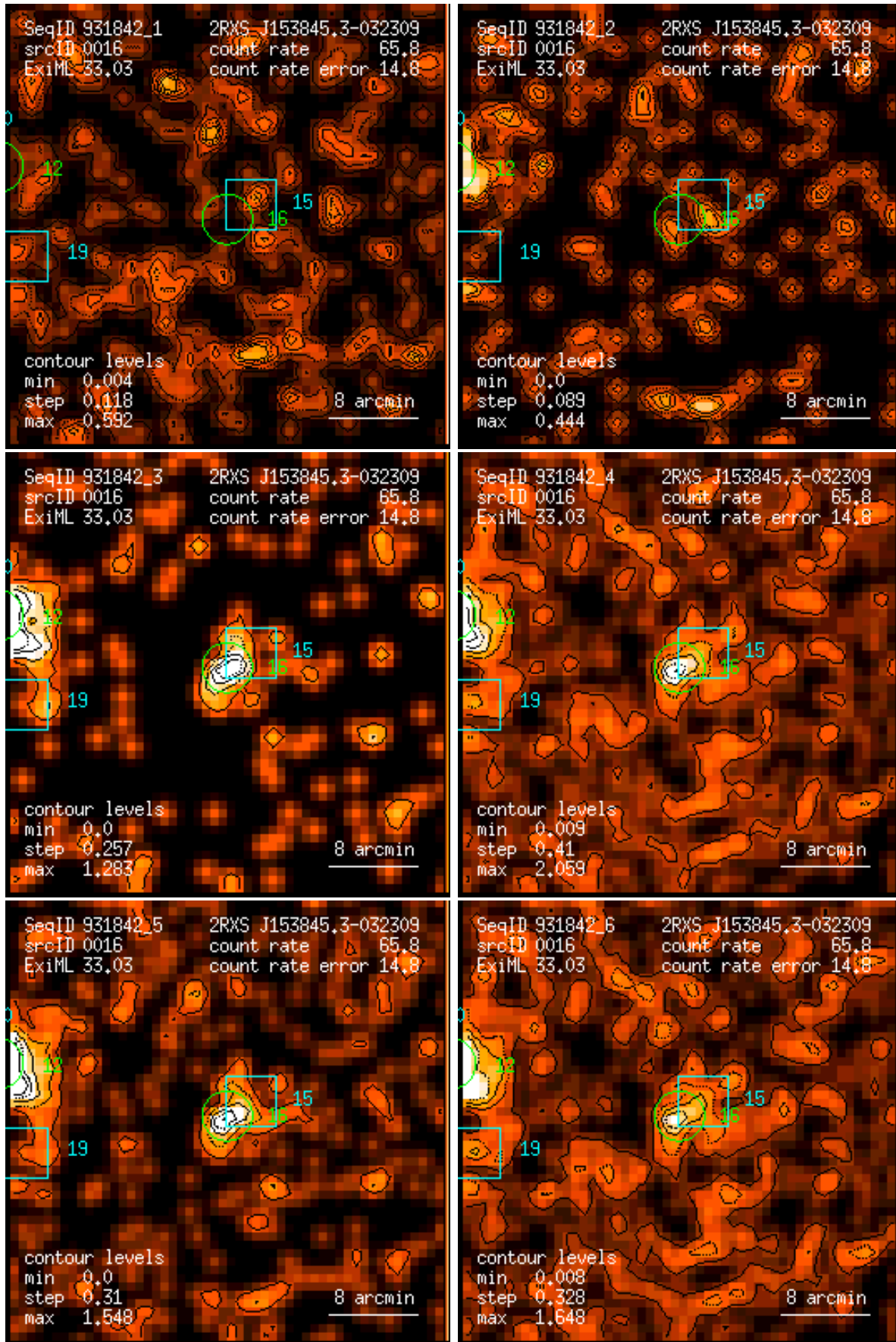
Figure 16: RASS 931842: detection 0016: band rate images, Gaussian filter: (1) PSPC channels 11 – 41, (2) 52 – 90, (3) 91 – 201, (4) 11 – 235, (5) 52 – 201, (6) 11 – 201. Broad band rates in counts/ks. Band rate contour levels in counts/ks/arcmin 2 .
