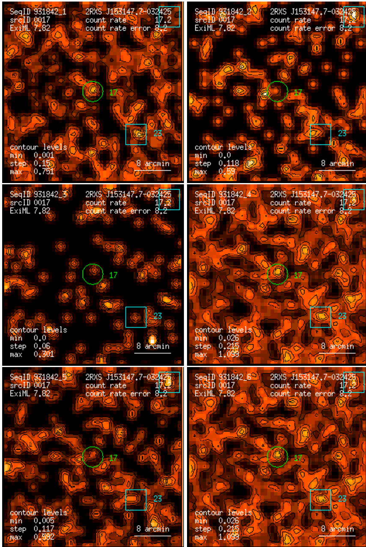
Figure 17: RASS 931842: detection 0017: band rate images, Gaussian filter: (1) PSPC channels 11 – 41, (2) 52 – 90, (3) 91 – 201, (4) 11 – 235, (5) 52 – 201, (6) 11 – 201. Broad band rates in counts/ks. Band rate contour levels in counts/ks/arcmin 2 .
