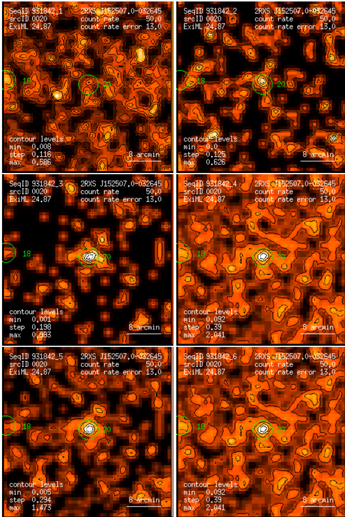
Figure 20: RASS 931842: detection 0020: band rate images, Gaussian filter: (1) PSPC channels 11 – 41, (2) 52 – 90, (3) 91 – 201, (4) 11 – 235, (5) 52 – 201, (6) 11 – 201. Broad band rates in counts/ks. Band rate contour levels in counts/ks/arcmin 2 .
