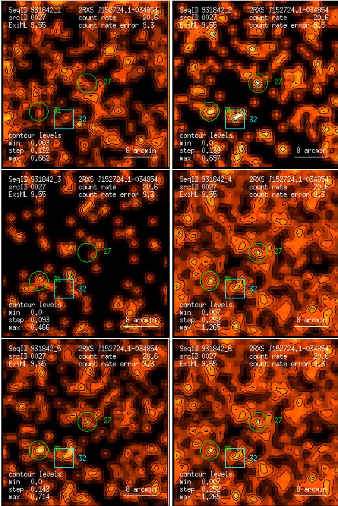
Figure 27: RASS 931842: detection 0027: band rate images, Gaussian filter: (1) PSPC channels 11 – 41, (2) 52 – 90, (3) 91 – 201, (4) 11 – 235, (5) 52 – 201, (6) 11 – 201. Broad band rates in counts/ks. Band rate contour levels in counts/ks/arcmin 2 .
