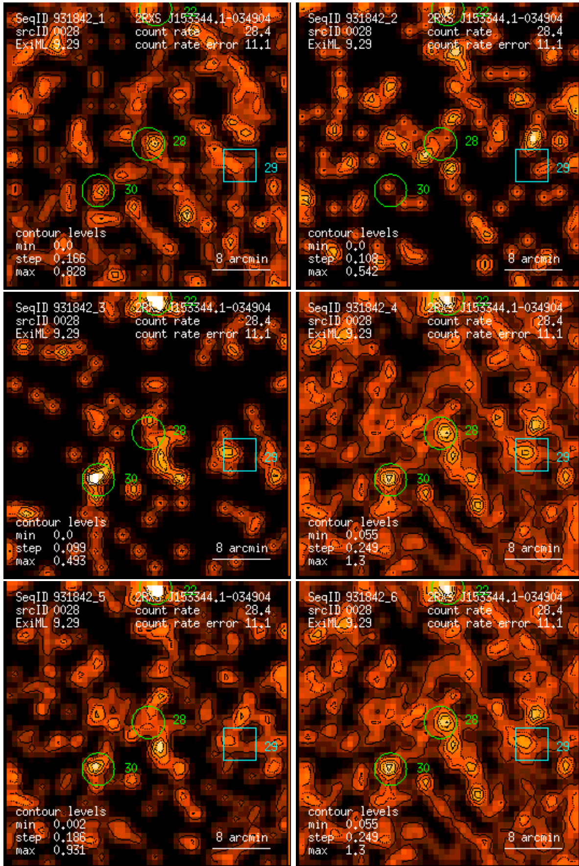
Figure 28: RASS 931842: detection 0028: band rate images, Gaussian filter: (1) PSPC channels 11 – 41, (2) 52 – 90, (3) 91 – 201, (4) 11 – 235, (5) 52 – 201, (6) 11 – 201. Broad band rates in counts/ks. Band rate contour levels in counts/ks/arcmin 2 .
