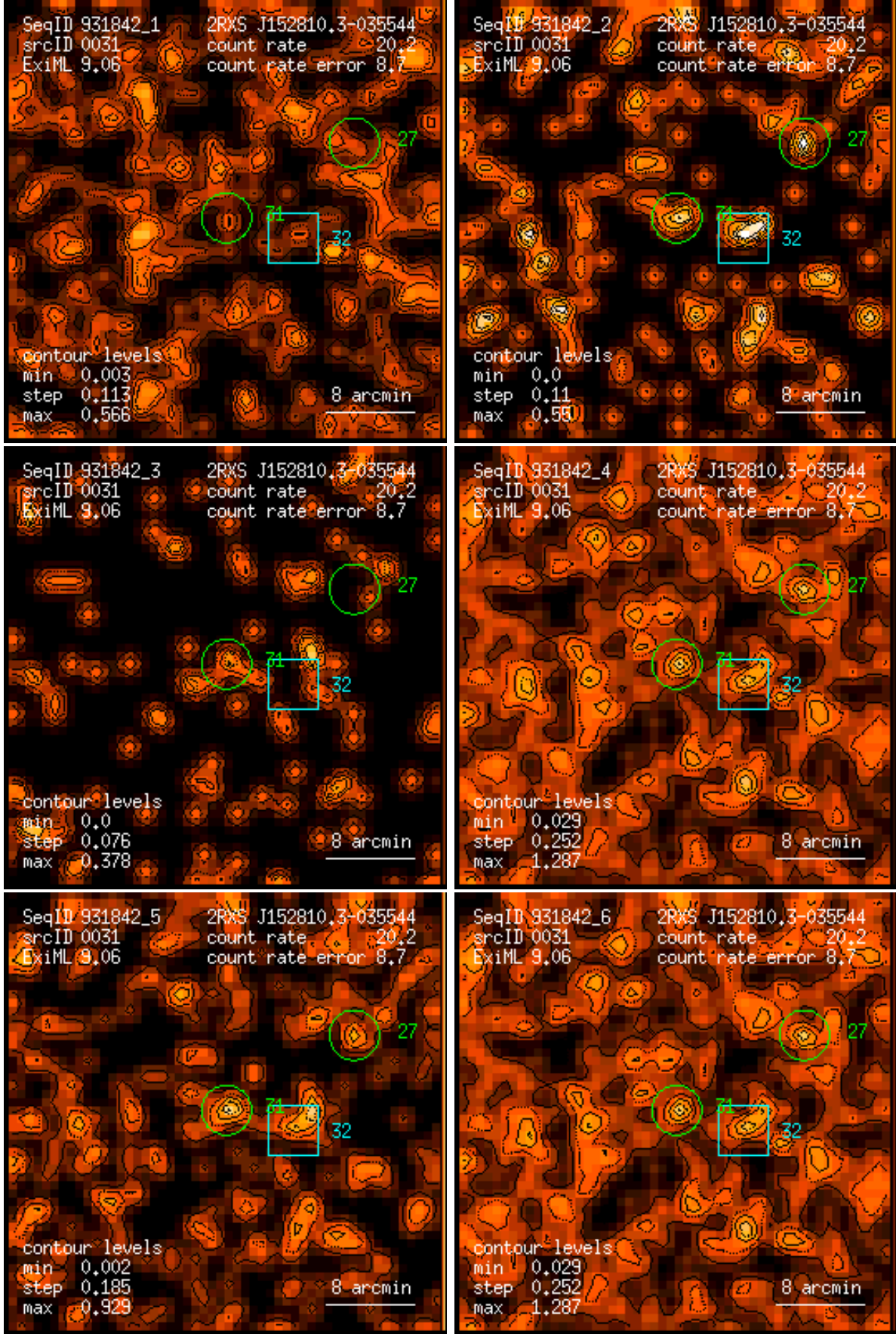
Figure 31: RASS 931842: detection 0031: band rate images, Gaussian filter: (1) PSPC channels 11 – 41, (2) 52 – 90, (3) 91 – 201, (4) 11 – 235, (5) 52 – 201, (6) 11 – 201. Broad band rates in counts/ks. Band rate contour levels in counts/ks/arcmin 2 .
