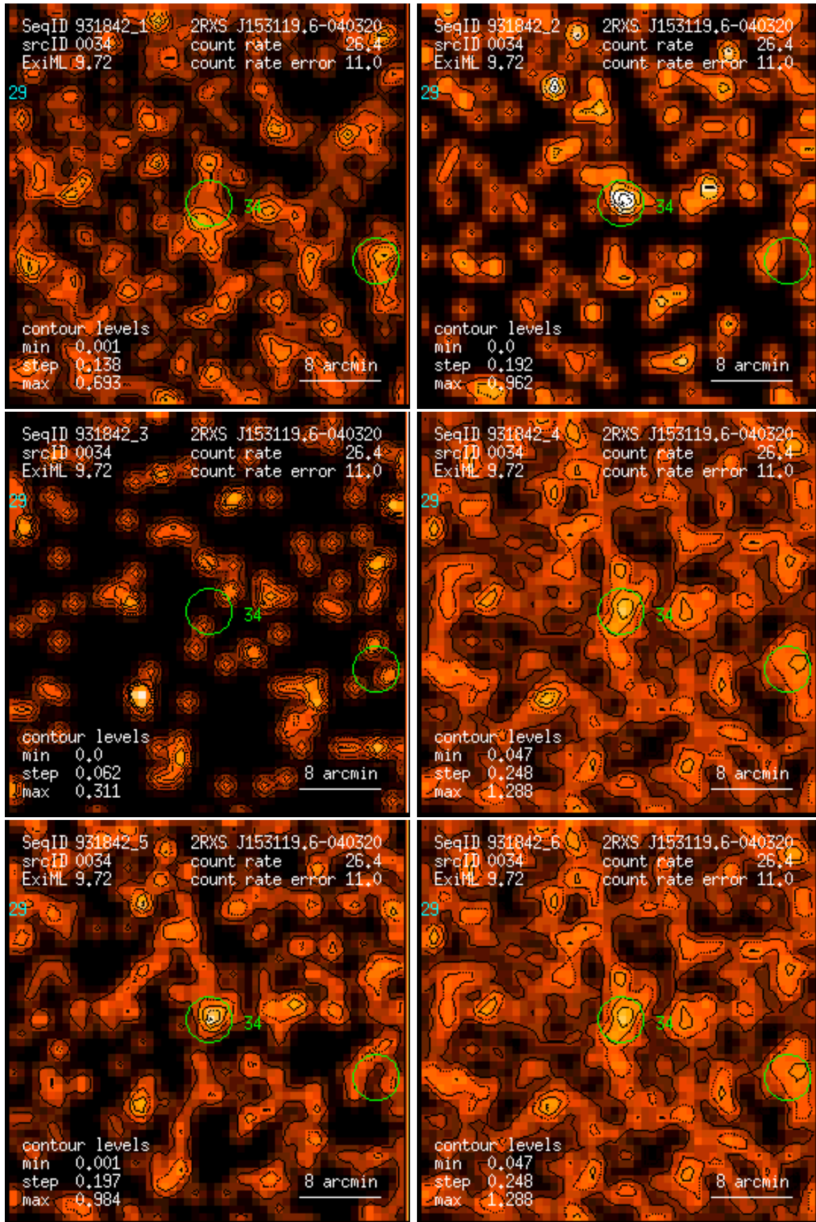
Figure 34: RASS 931842: detection 0034: band rate images, Gaussian filter: (1) PSPC channels 11 – 41, (2) 52 – 90, (3) 91 – 201, (4) 11 – 235, (5) 52 – 201, (6) 11 – 201. Broad band rates in counts/ks. Band rate contour levels in counts/ks/arcmin 2 .
