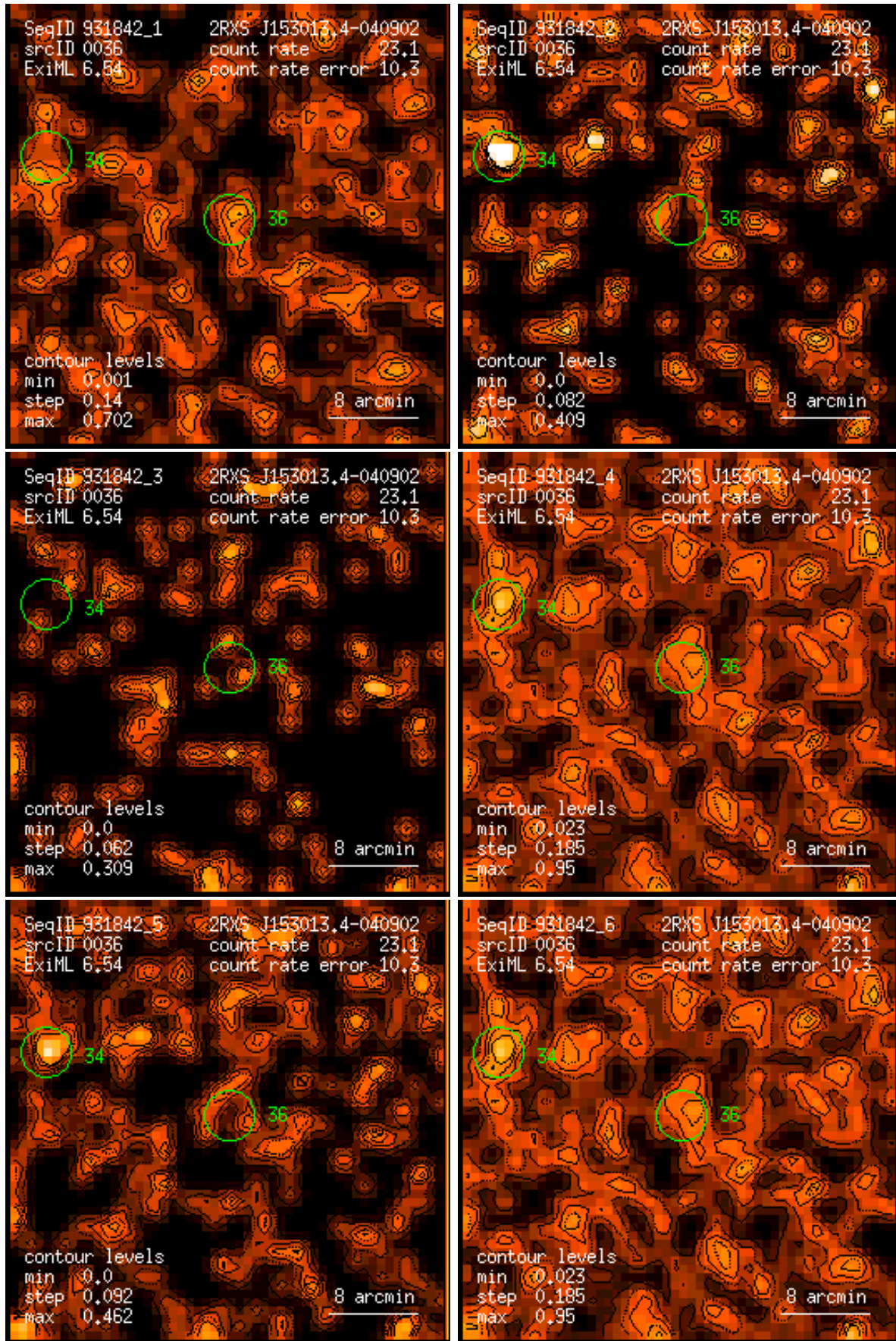
Figure 36: RASS 931842: detection 0036: band rate images, Gaussian filter: (1) PSPC channels 11 – 41, (2) 52 – 90, (3) 91 – 201, (4) 11 – 235, (5) 52 – 201, (6) 11 – 201. Broad band rates in counts/ks. Band rate contour levels in counts/ks/arcmin 2 .
