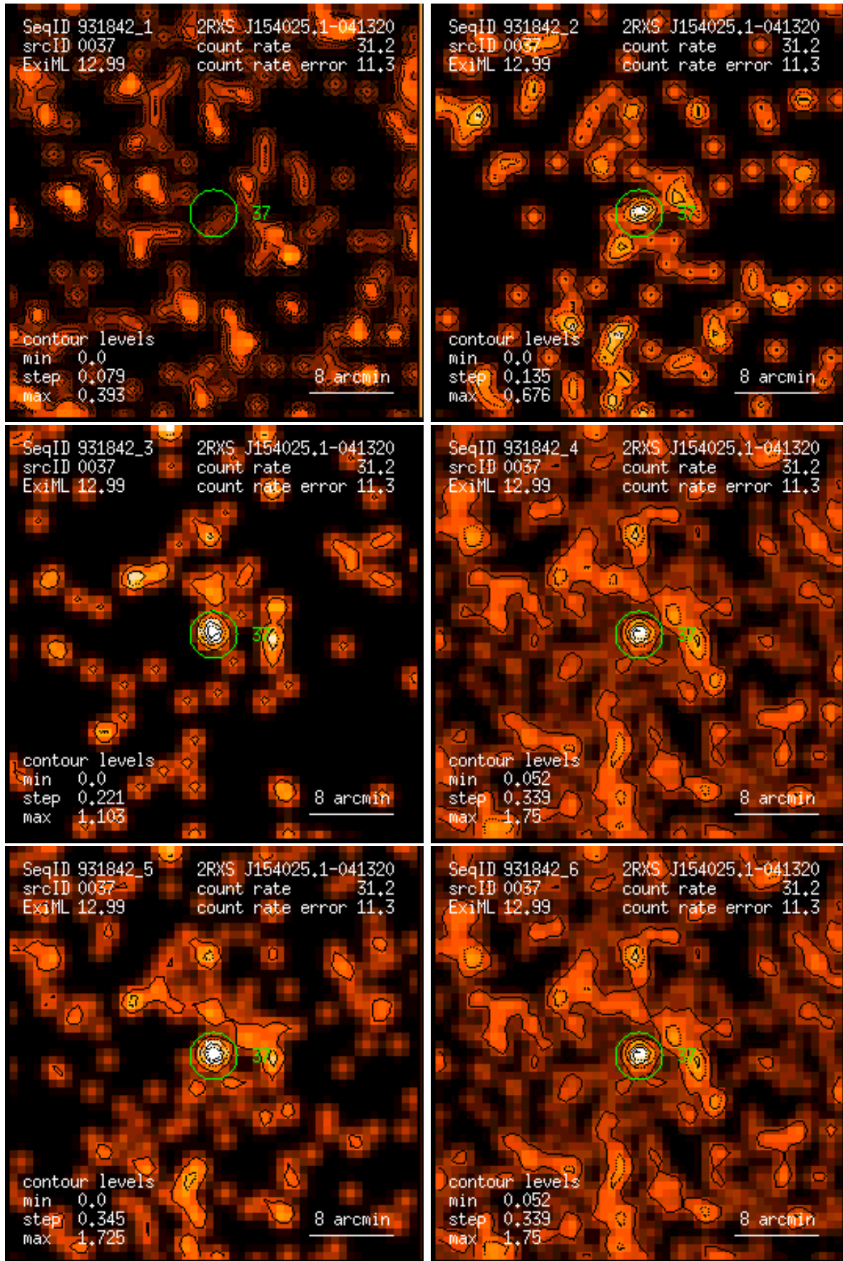
Figure 37: RASS 931842: detection 0037: band rate images, Gaussian filter: (1) PSPC channels 11 – 41, (2) 52 – 90, (3) 91 – 201, (4) 11 – 235, (5) 52 – 201, (6) 11 – 201. Broad band rates in counts/ks. Band rate contour levels in counts/ks/arcmin 2 .
