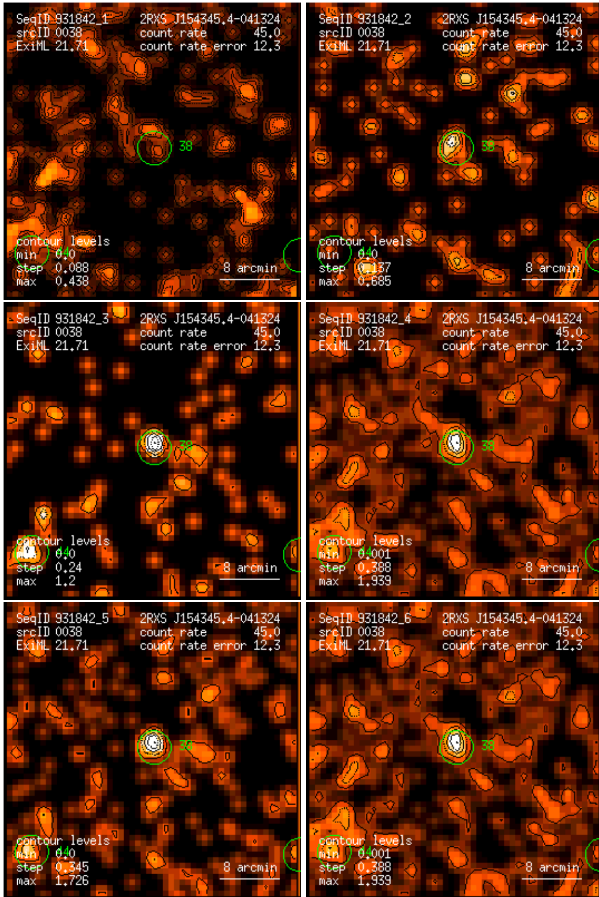
Figure 38: RASS 931842: detection 0038: band rate images, Gaussian filter: (1) PSPC channels 11 – 41, (2) 52 – 90, (3) 91 – 201, (4) 11 – 235, (5) 52 – 201, (6) 11 – 201. Broad band rates in counts/ks. Band rate contour levels in counts/ks/arcmin 2 .
