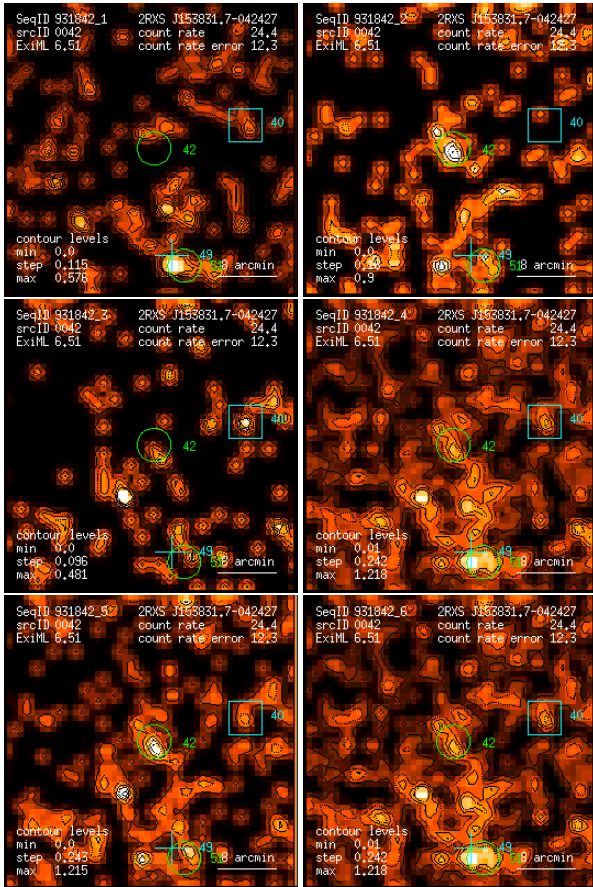
Figure 42: RASS 931842: detection 0042: band rate images, Gaussian filter: (1) PSPC channels 11 – 41, (2) 52 – 90, (3) 91 – 201, (4) 11 – 235, (5) 52 – 201, (6) 11 – 201. Broad band rates in counts/ks. Band rate contour levels in counts/ks/arcmin 2 .
